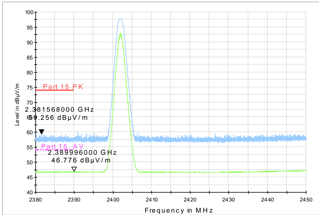
RE - Power-2.38GHz-2.45GHz
