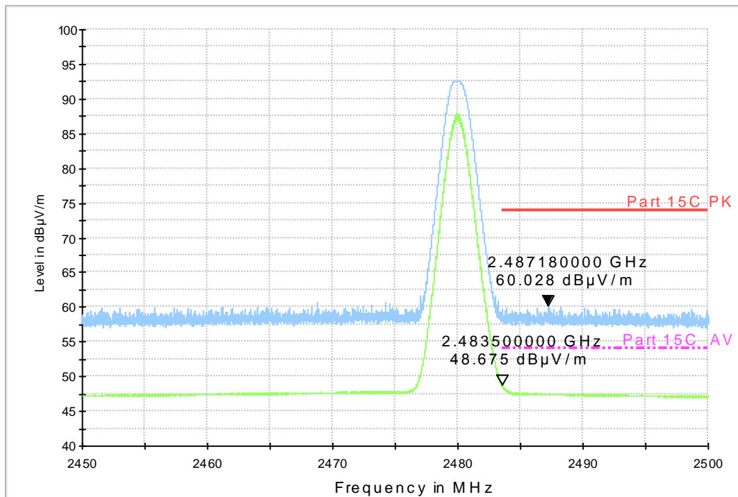
Fig.19. Transmitter Spurious Emission - Radiated (Power): GFSK high channel
