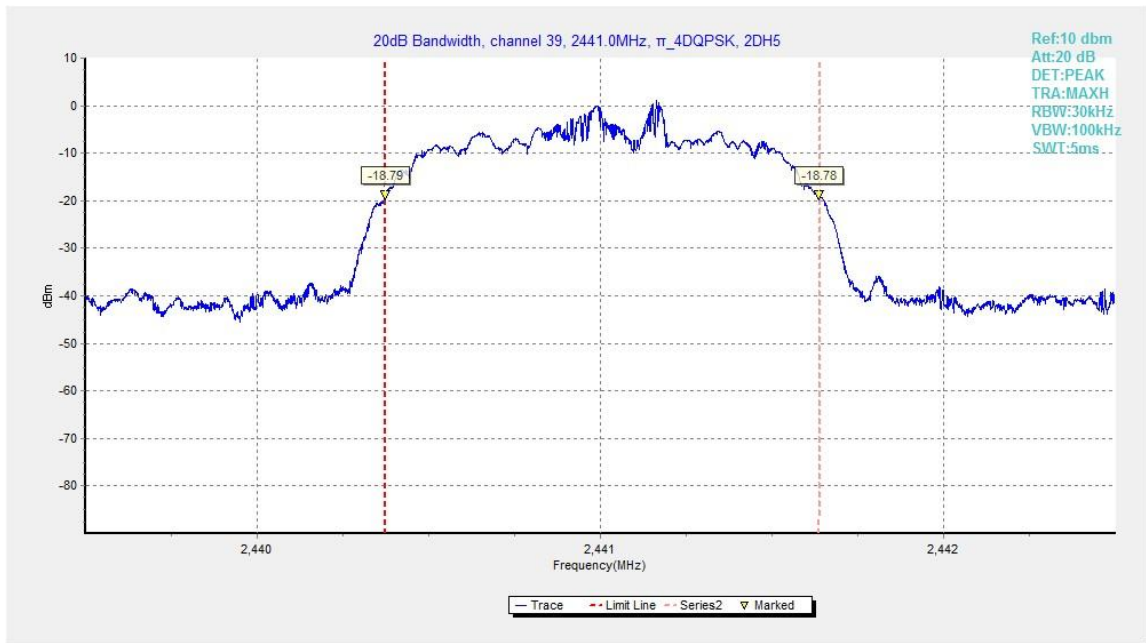
Fig.85. 20dB Bandwidth: \pi/4 DQPSK, Channel 39
