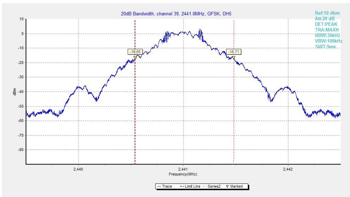
Fig.82. 20dB Bandwidth: GFSK, Channel 39
