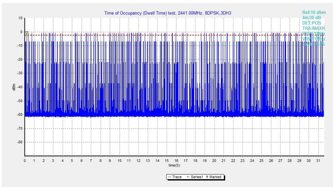
Fig.78. Number of Transmissions Measurement: Channel 39,Packet 3-DH3
