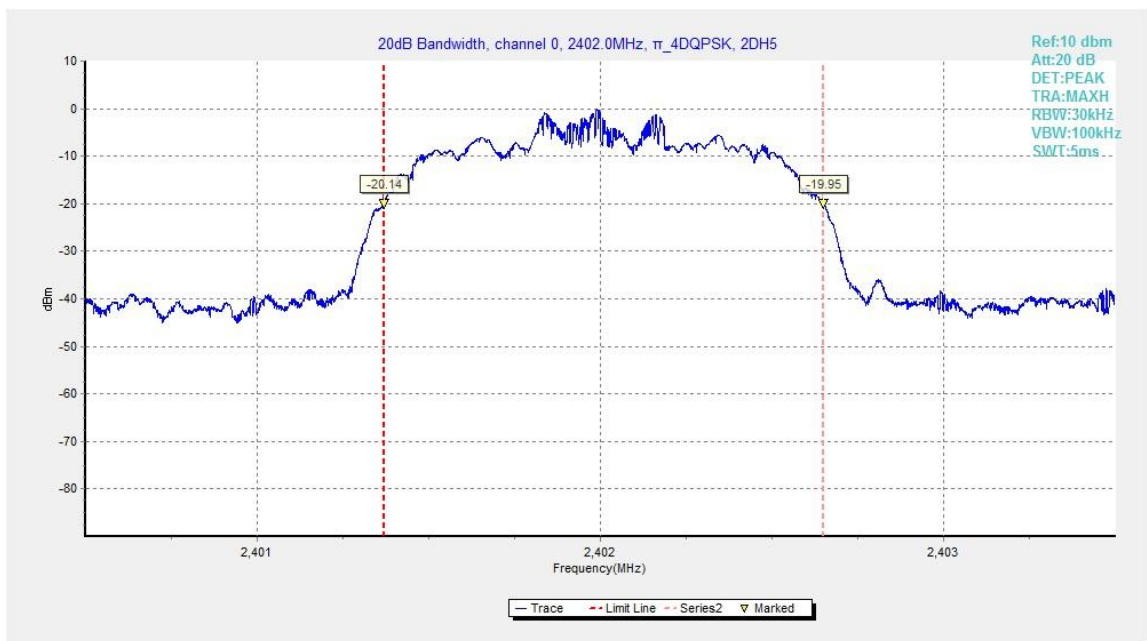
Fig.84. 20dB Bandwidth: \pi/4 DQPSK, Channel 0
