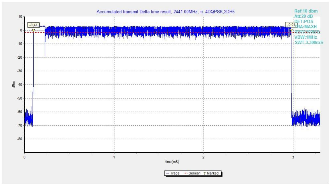
Fig.73. Time of occupancy (Dwell Time): Channel 39, Packet 2-DH5
