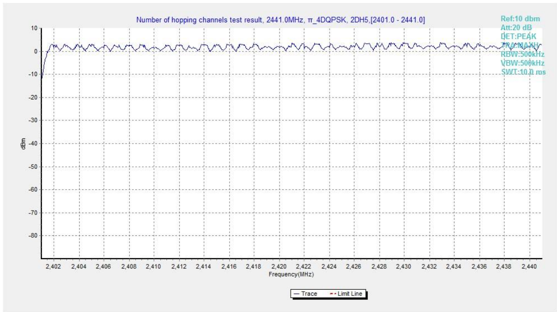
Fig.95. Number of hopping frequencies: \pi/4 DQPSK, Channel 0 - 39
