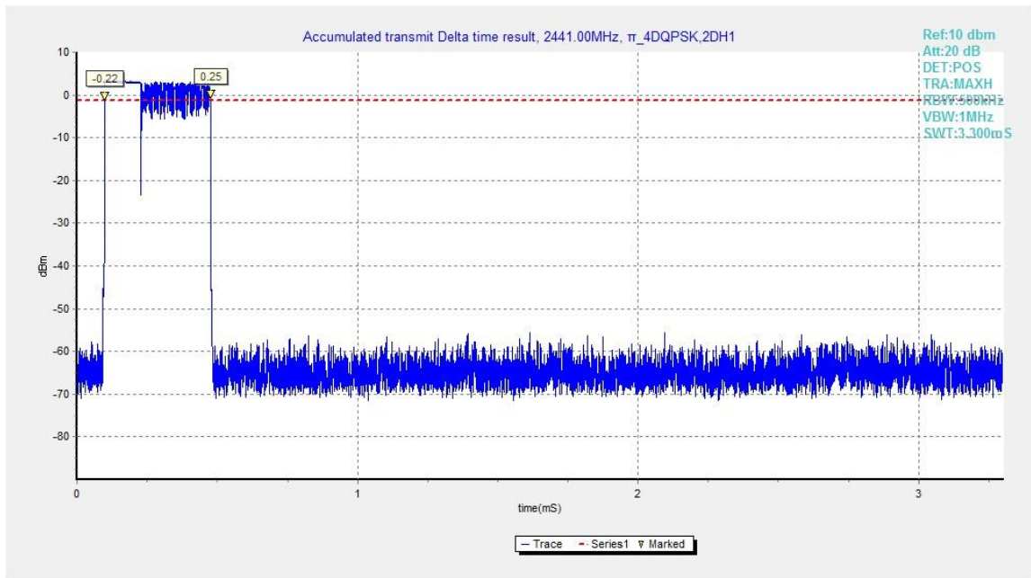
Fig.69. Time of occupancy (Dwell Time): Channel 39, Packet 2-DH1
