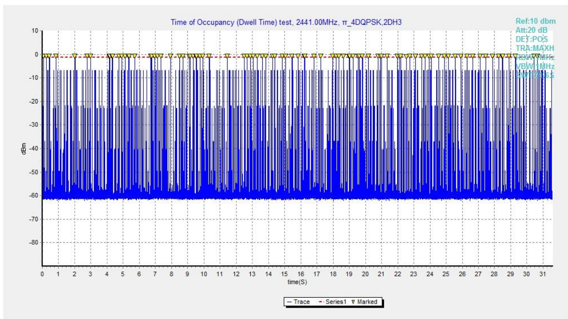
Fig.72. Number of Transmissions Measurement: Channel 39,Packet 2-DH3
