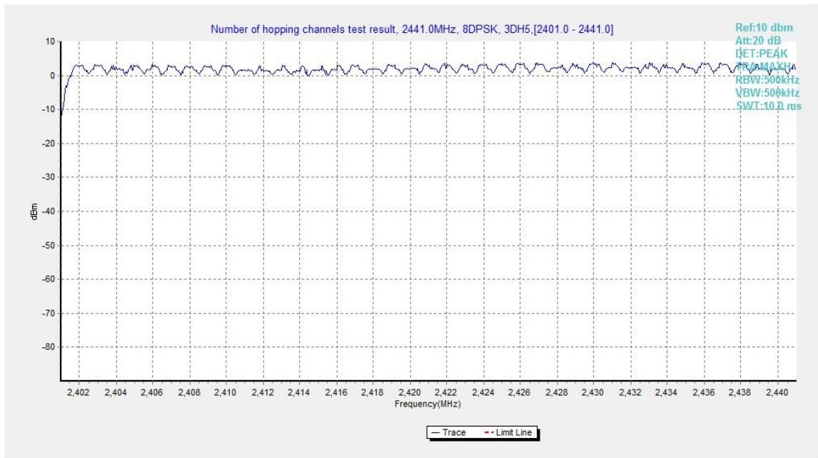
Fig.97. Number of hopping frequencies: 8DPSK, Channel 0 - 39
