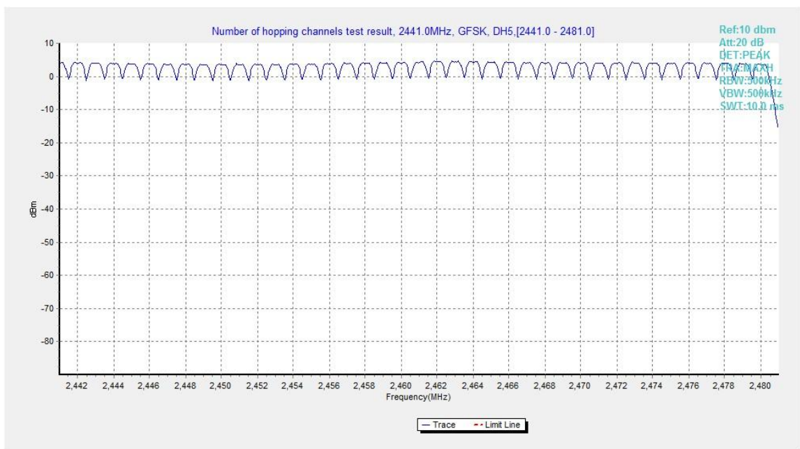
Fig.94. Number of hopping frequencies: GFSK, Channel 40 - 78
