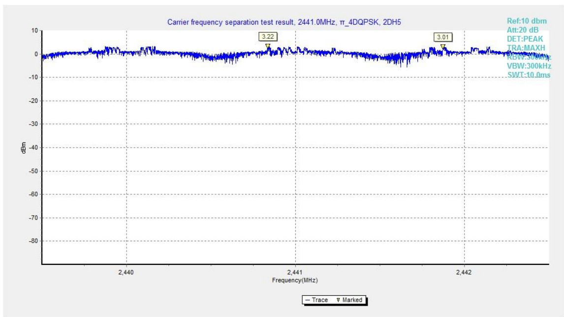
Fig.91. Carrier frequency separation measurement: \pi/4 DQPSK, Channel 39
