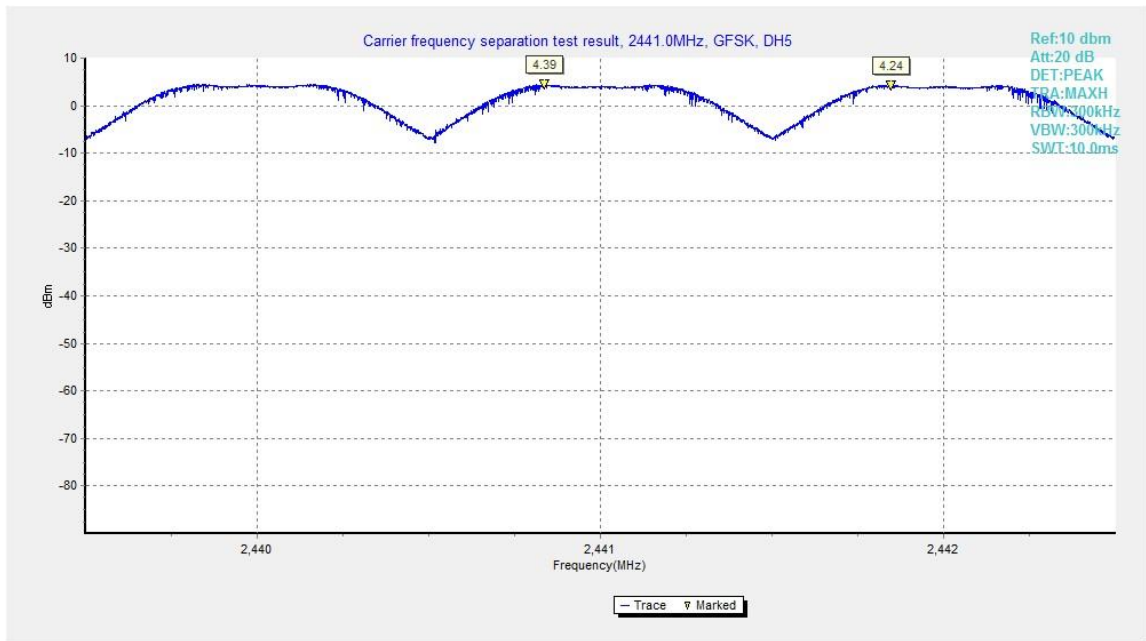
Fig.90. Carrier frequency separation measurement: GFSK, Channel 39
