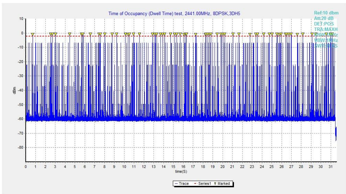
Fig.80. Number of Transmissions Measurement: Channel 39,Packet 3-DH5
