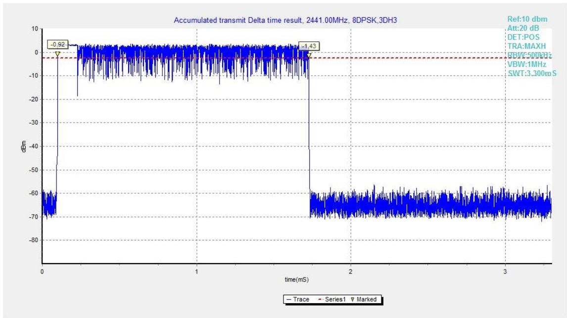
Fig.77. Time of occupancy (Dwell Time): Channel 39, Packet 3-DH3
