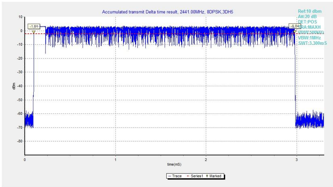
Fig.79. Time of occupancy (Dwell Time): Channel 39, Packet 3-DH5
