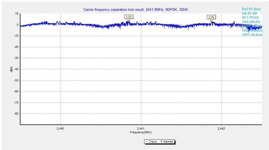
Fig.92. Carrier frequency separation measurement: 8DPSK, Channel 39
