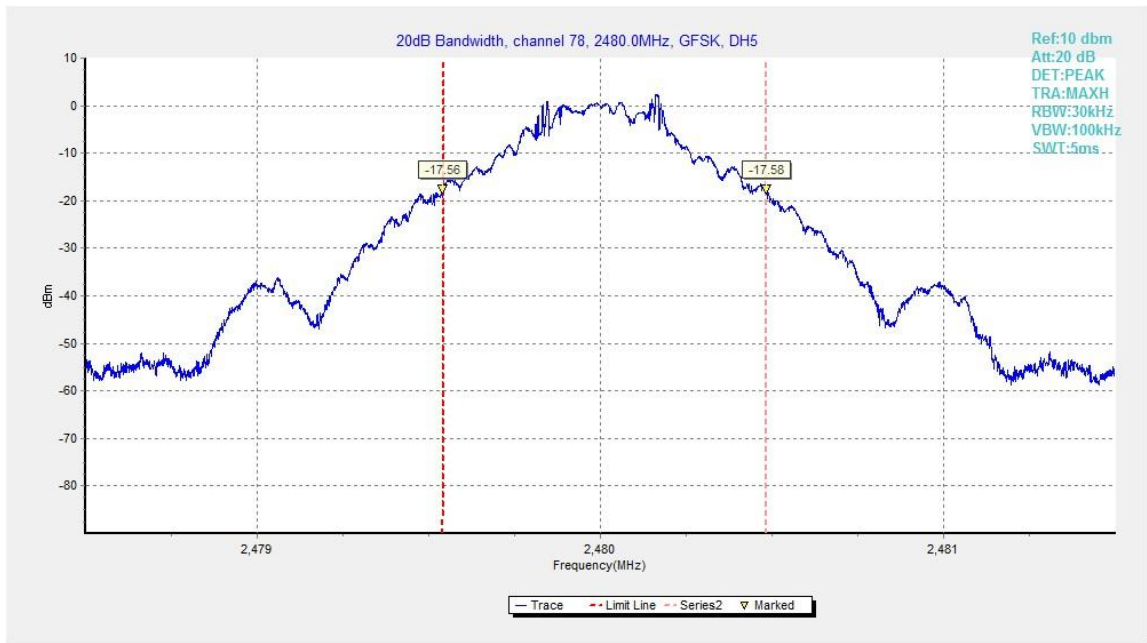
Fig.83. 20dB Bandwidth: GFSK, Channel 78
