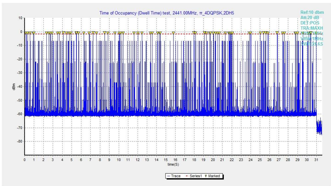
Fig.74. Number of Transmissions Measurement: Channel 39,Packet 2-DH5
