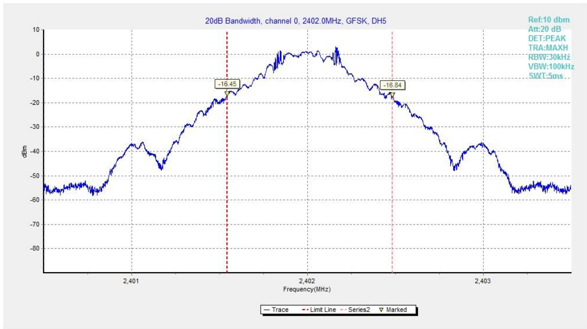
Fig.81. 20dB Bandwidth: GFSK, Channel 0
