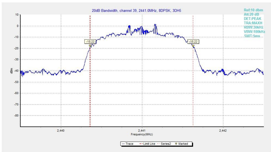
Fig.88. 20dB Bandwidth: 8DPSK, Channel 39
