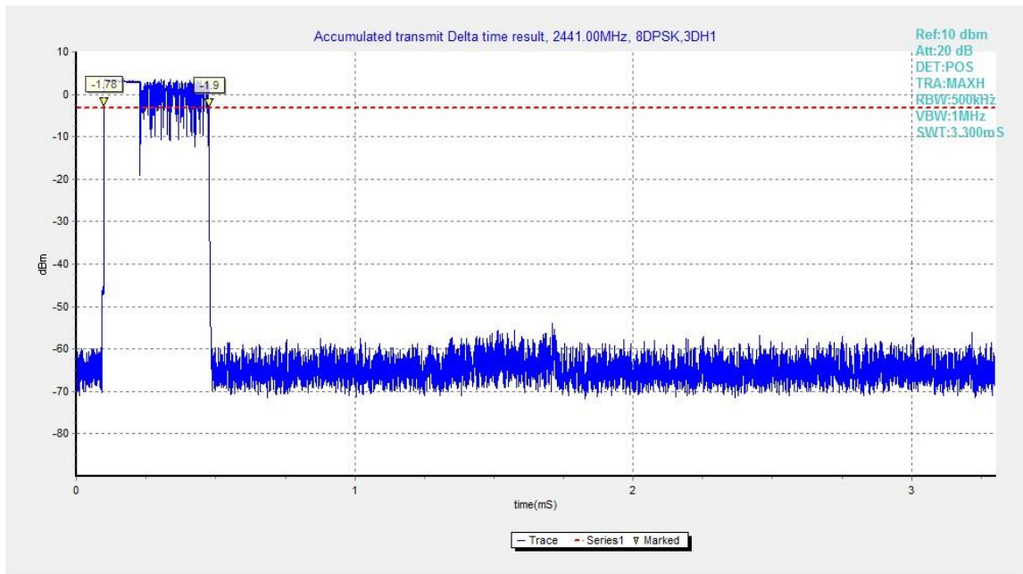
Fig.75. Time of occupancy (Dwell Time): Channel 39, Packet 3-DH1
