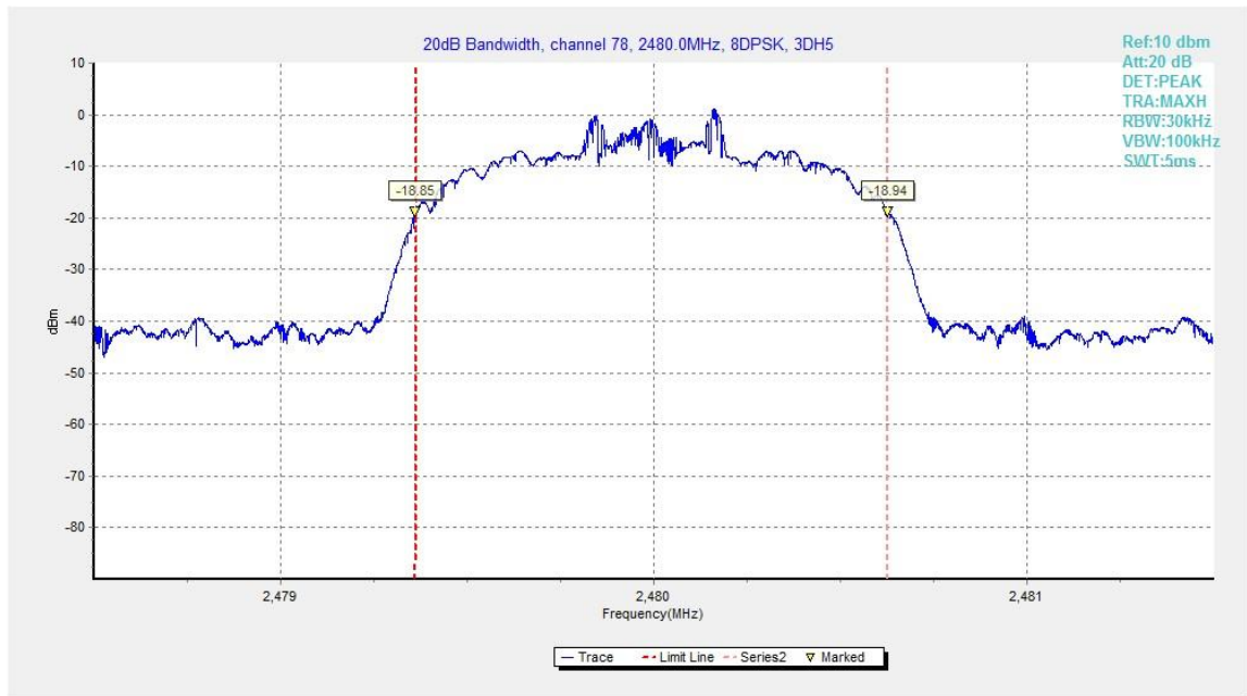
Fig.89. 20dB Bandwidth: 8DPSK, Channel 78
