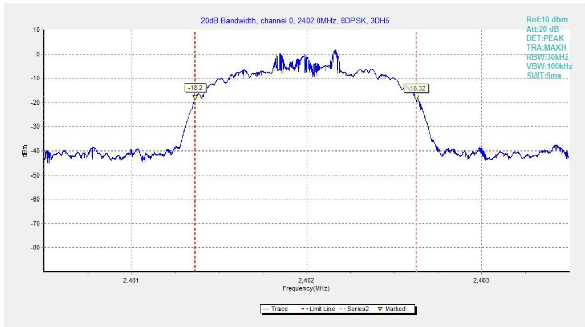
Fig.87. 20dB Bandwidth: 8DPSK, Channel 0
