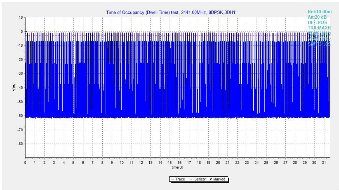
Fig.76. Number of Transmissions Measurement: Channel 39,Packet 3-DH1
