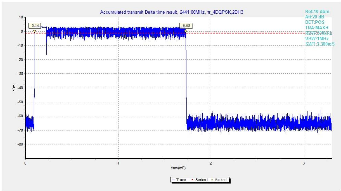
Fig.71. Time of occupancy (Dwell Time): Channel 39, Packet 2-DH3
