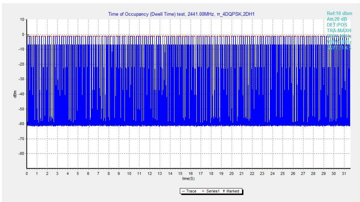
Fig.70. Number of Transmissions Measurement: Channel 39,Packet 2-DH1
