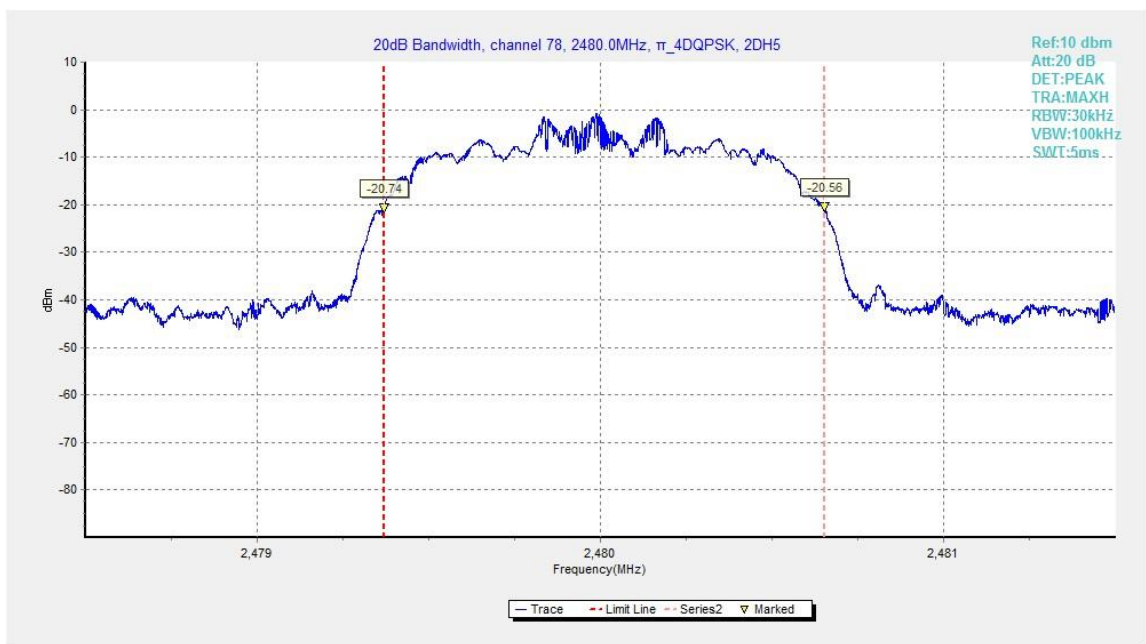
Fig.86. 20dB Bandwidth: \pi/4 DQPSK, Channel 78
