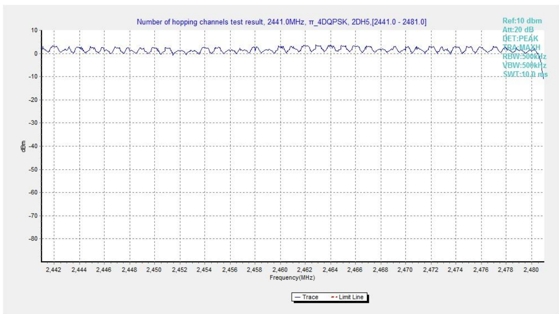
Fig.96. Number of hopping frequencies: \pi/4 DQPSK, Channel 40 - 78
