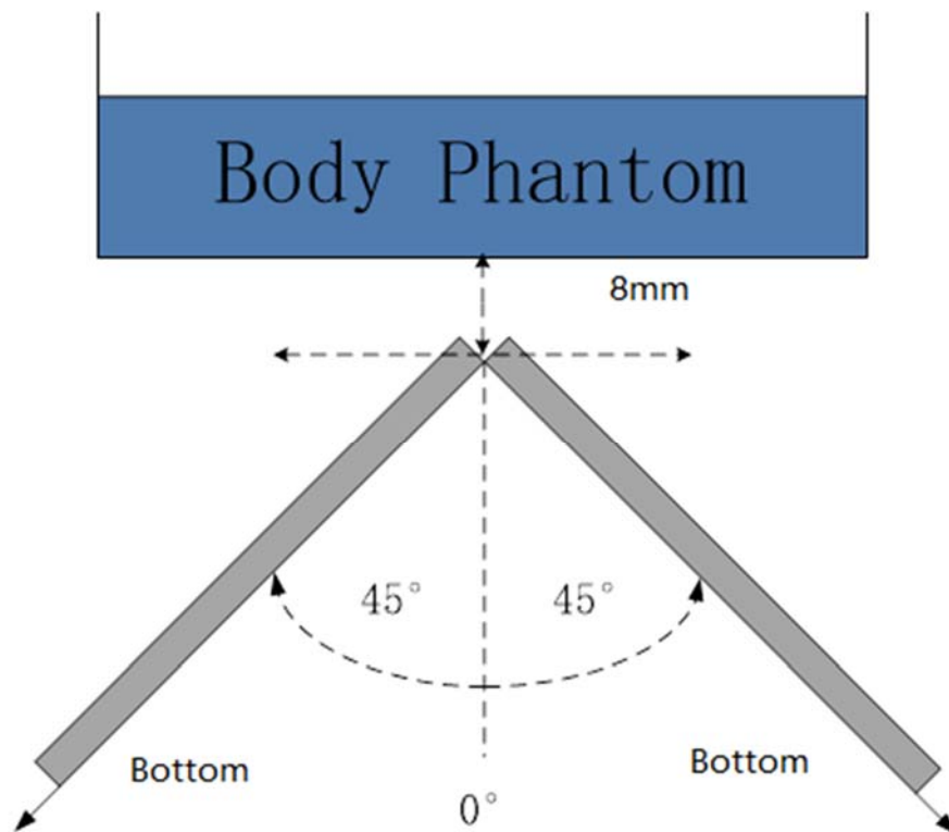
The bottom edge evaluation for main antenna
