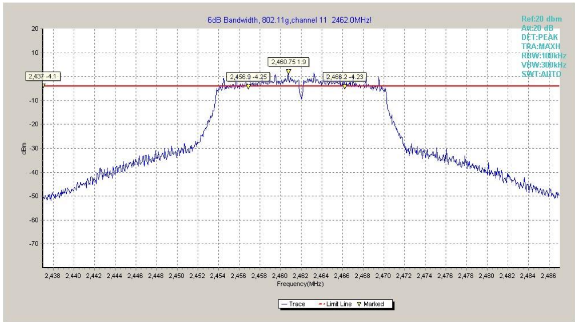
Fig.A.4.6 Occupied 6dB Bandwidth (802.11g, Ch 11)
