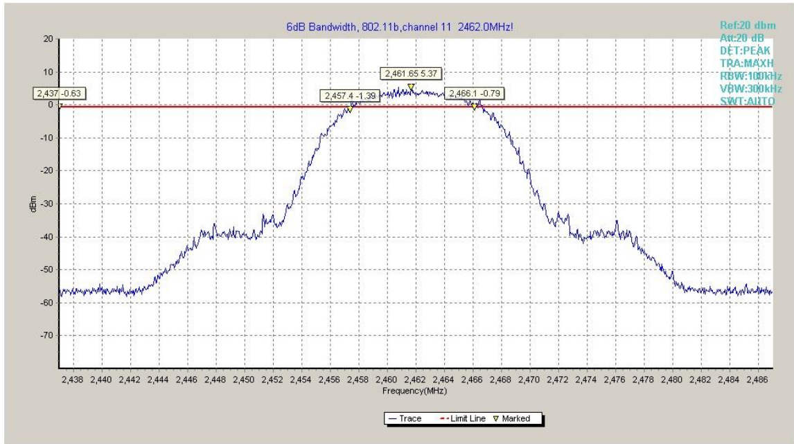
Fig.A.4.3 Occupied 6dB Bandwidth (802.11b, Ch 11)
