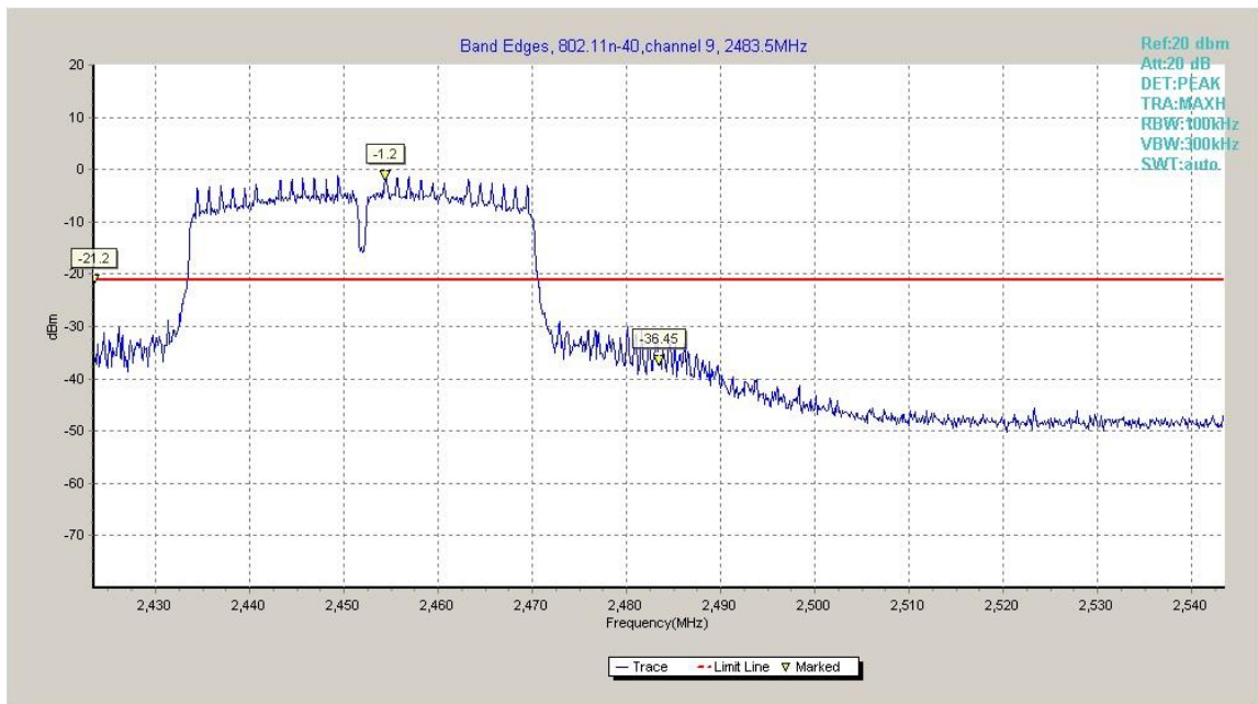
Fig.A.5.8 Band Edges (802.11n-HT40, Ch 9)
