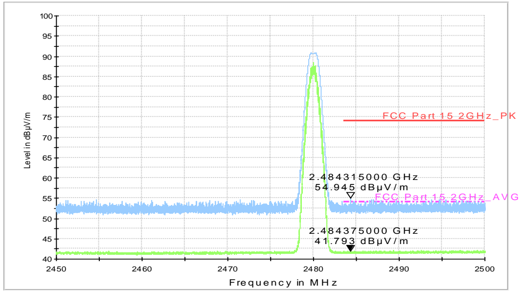
Fig.19. Transmitter Spurious Emission - Radiated (Power): GFSK high channel
