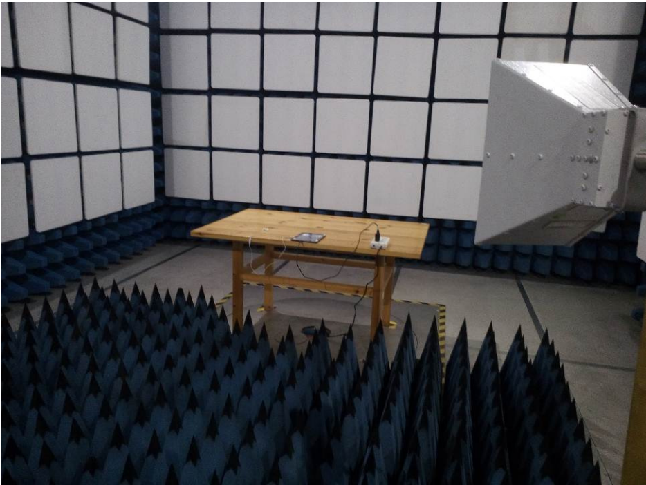
Above 1 GHz Back video record mode (C-P35 Acbel Charger)
