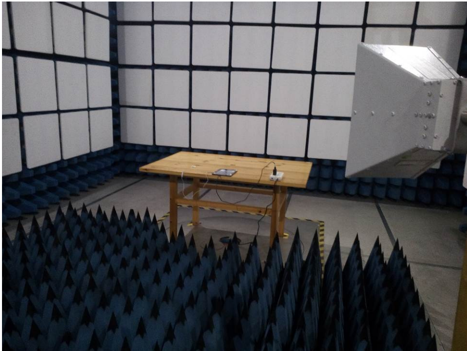
Above 1 GHz Back video record mode (C-P35 Hunktey Charger)
