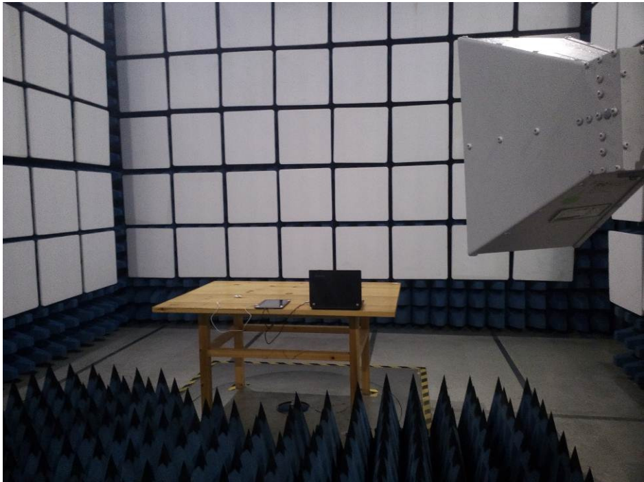
Above 1 GHz (Download mode)
