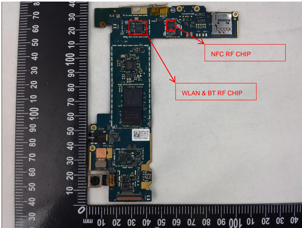
Mainboard front view without shielding
