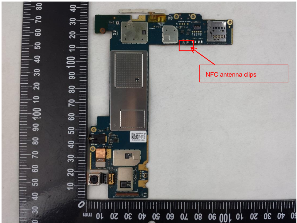
Mainboard front view with shielding
