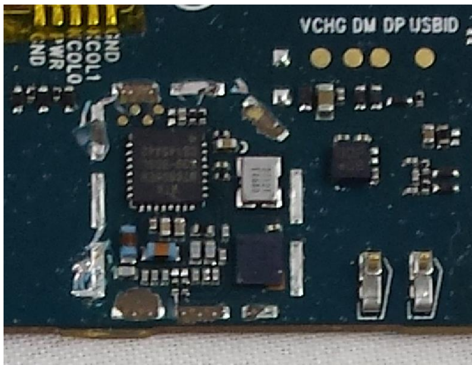
NFC RF section view
