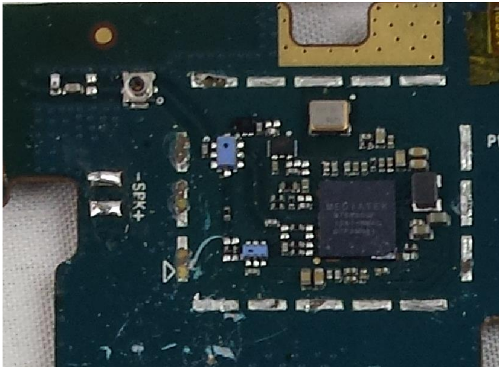
WLAN & BT RF section view
