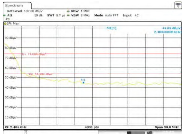
802.11n-20 HIGH CHANNEL , PEAK
