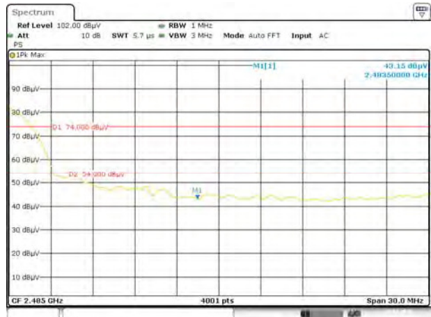
802.11g HIGH CHANNEL , PEAK
