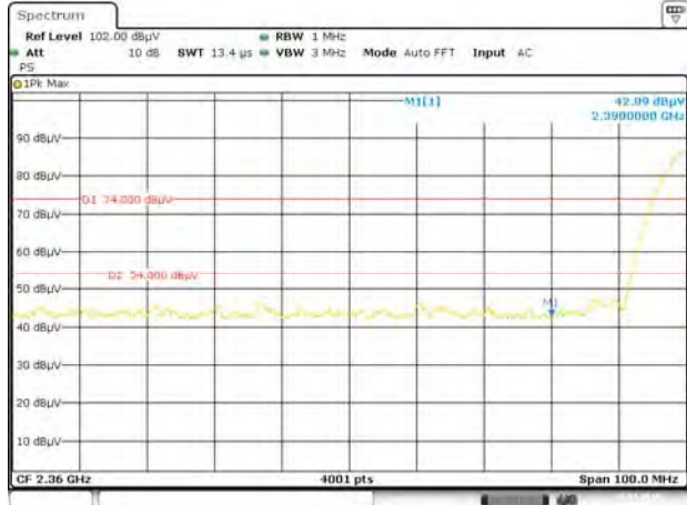
802.11b LOW CHANNEL , PEAK
