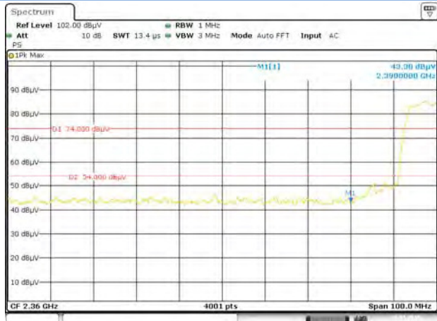
802.11n-20 LOW CHANNEL , PEAK
