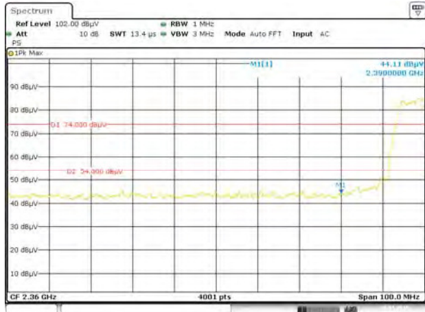
802.11g LOW CHANNEL , PEAK
