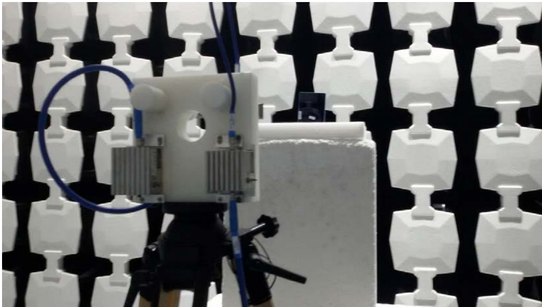
Description: Radiated Emission Test Setup (Above 18GHz)
