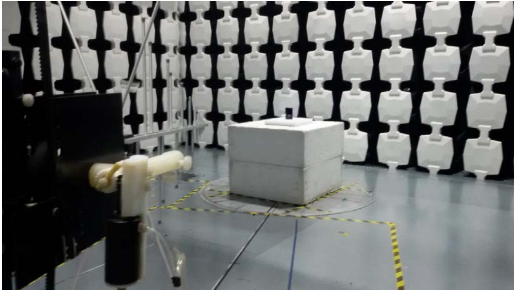
Description: Radiated Emission Test Setup (30-1000MHz)
