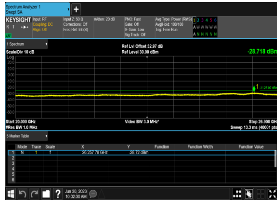
N41(30M)_DFT-s-OFDM_QPSK_Edge_1RB_Left_Mid_CH
