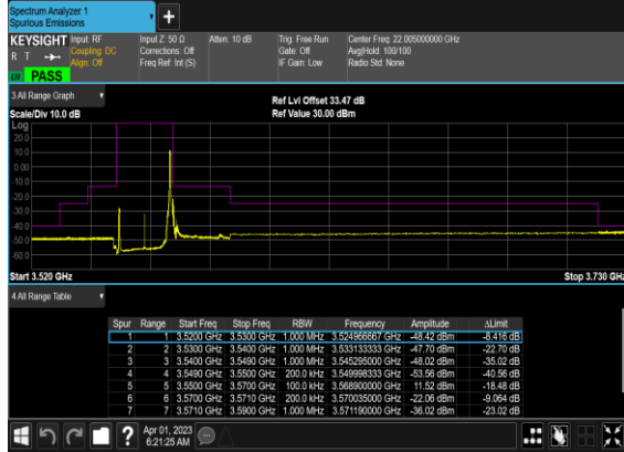
N78(20M)_DFT-s-OFDM_BPSK_Edge_1RB_Right_Low_CH
