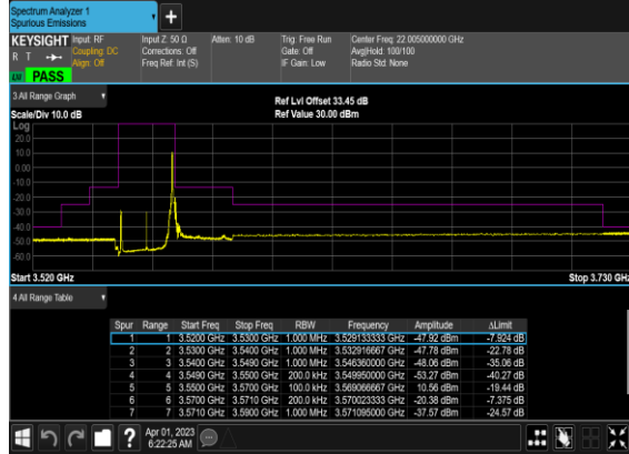
N78(20M)_DFT-s-OFDM_QPSK_Edge_1RB_Right_Low_CH
