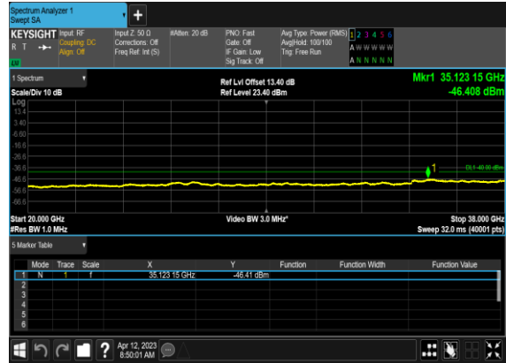
N78(60M)_DFT-s-OFDM_QPSK_Edge_1RB_Left_Mid_CH
