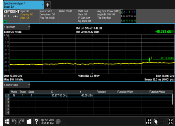
N78(60M)_DFT-s-OFDM_BPSK_Edge_1RB_Left_High_CH
