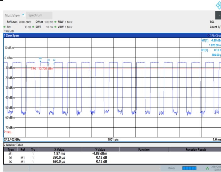
BLE_1M_Ant4_2402
