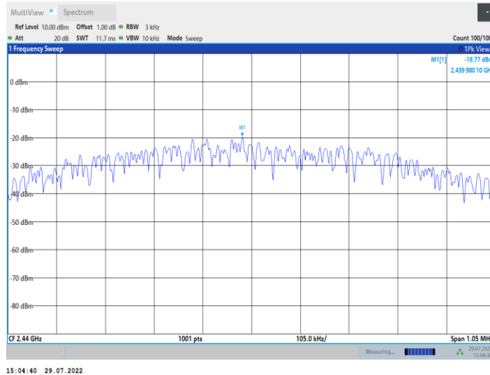
BLE_1M_Ant4_2440
