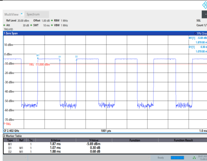
BLE_2M_Ant4_2402
