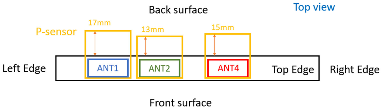
Photograph 25. Antenna position of EUT
