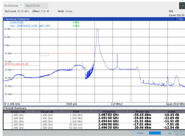
Band41-5MHz-QPSK-39675-25RB#0
