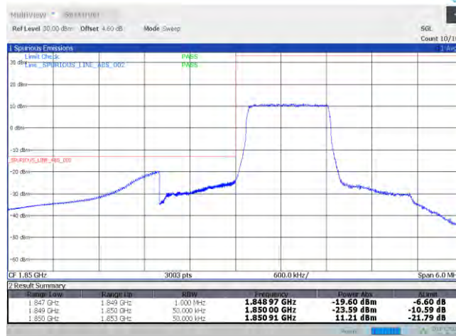
Band2-1.4MHz-QPSK-18607-6RB#0
