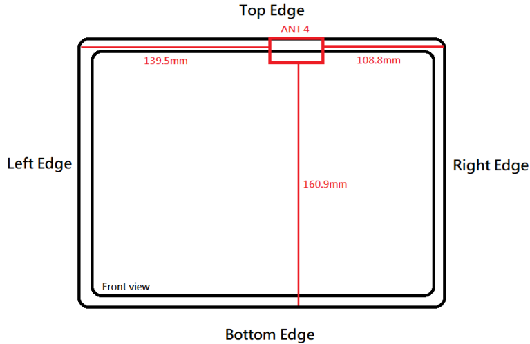
Photograph 21. Antenna position of EUT
