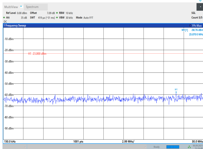
Band17-10MHz-QPSK-23780-1RB#0-Range2:0.15~30MHz
