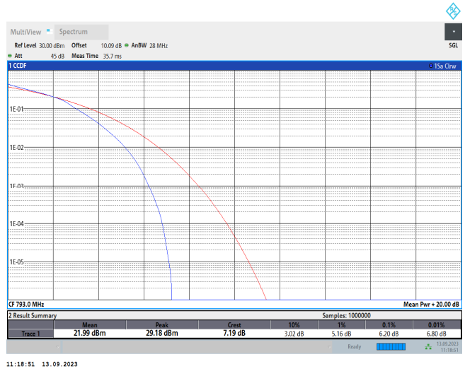
Band14-10MHz-16QAM-23330-50RB#0
