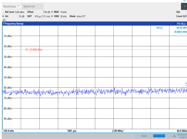
Band5-10MHz-QPSK-20450-1RB#0-Range2:0.15~30MHz
