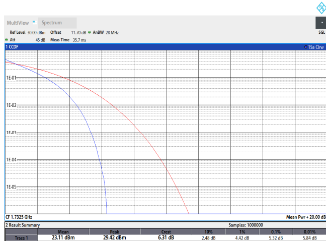
Band4-20MHz-QPSK-20175-100RB#0
