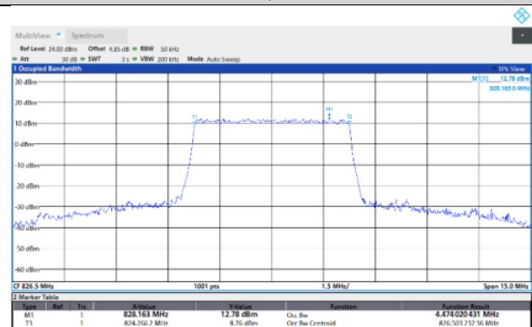
Band26-5MHz-16QAM-26815-25RB#0
