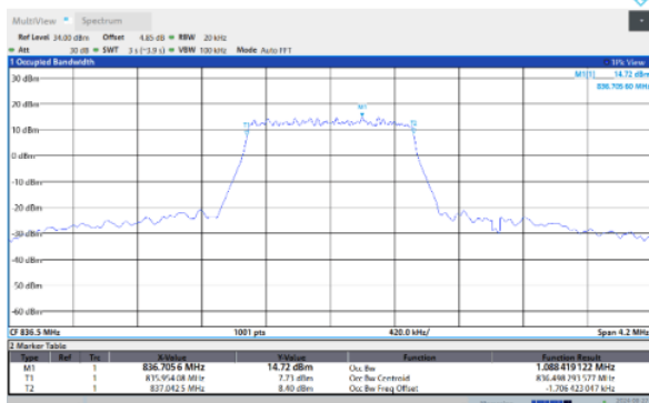
Band26-1.4MHz-64QAM-26797-6RB#0
