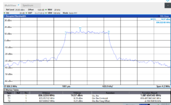
Band26-1.4MHz-64QAM-26915-6RB#0
