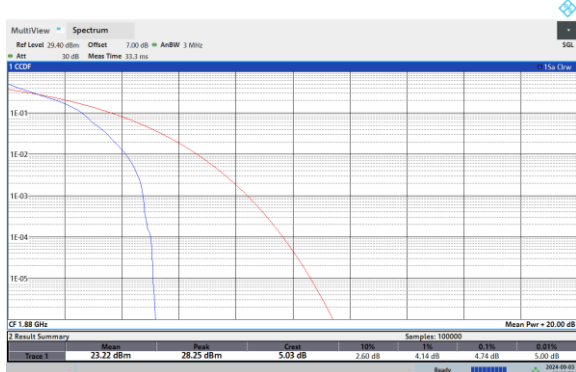
Band25-3MHz-QPSK-26675-1RB#0
