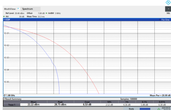
Band25-3MHz-QPSK-26675-15RB#0
