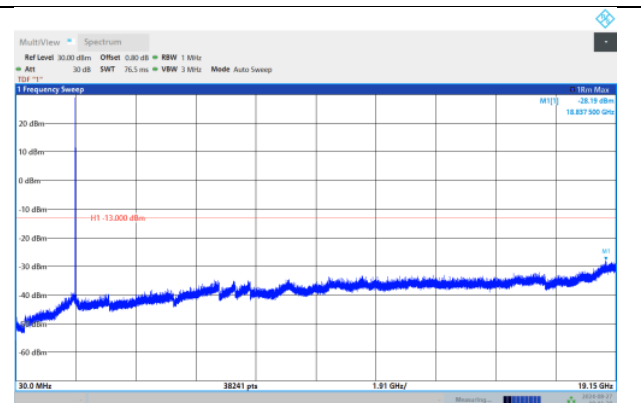
Band25-1.4MHz-64QAM-26340-1RB#0- Range:30~19150
