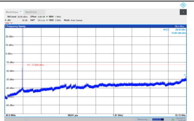
Band25-3MHz-QPSK-26675-1RB#0-Range:30~19150
