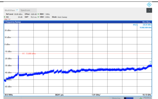
Band25-20MHz-QPSK-26140-1RB#0- Range:30~19150
