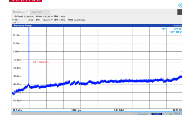
Band25-1.4MHz-64QAM-26047-1RB#0- Range:30~19150
