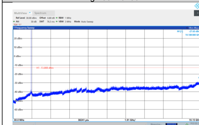
Band25-1.4MHz-64QAM-26683-1RB#0- Range:30~19150
