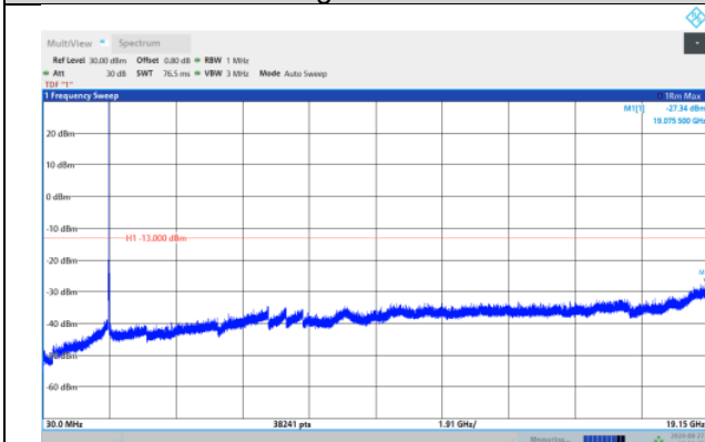
Band25-10MHz-64QAM-26340-1RB#0- Range:30~19150
