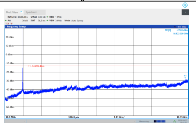
Band25-20MHz-16QAM-26340-1RB#0- Range:30~19150
