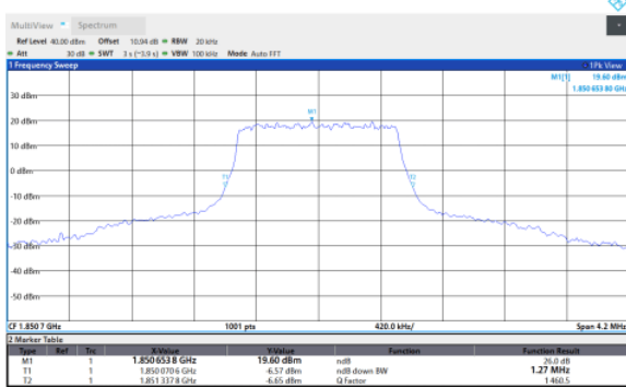
Band25-1.4MHz-QPSK-26683-6RB#0
