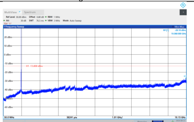
Band25-10MHz-64QAM-26090-1RB#0- Range:30~19150
