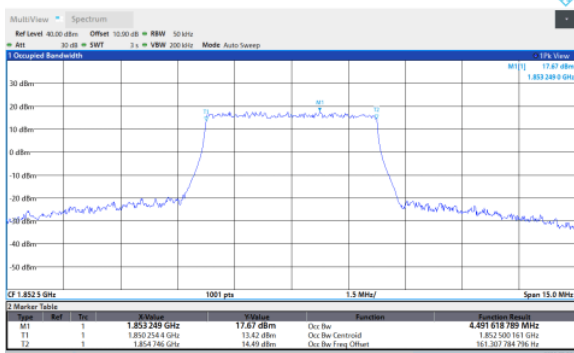
Band25-5MHz-QPSK-26665-25RB#0
