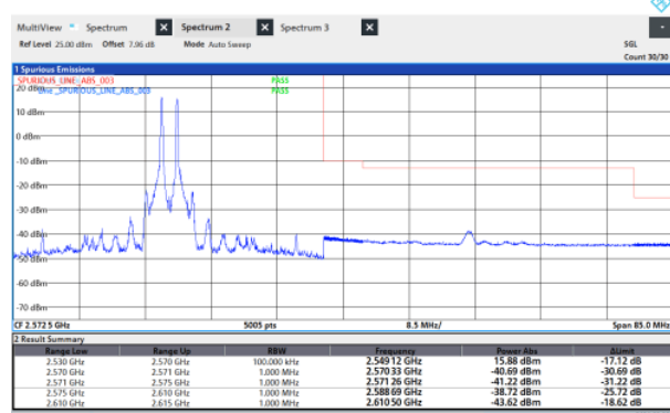
7-7-20MHz-20MHz-64QAM-64QAM-21152-21350-21048-1RB#99-1RB#0
