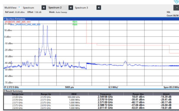
7-7-20MHz-20MHz-64QAM-64QAM-20850-21048-21048-1RB#0-1RB#99
