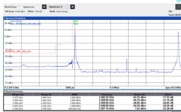
7-7-20MHz-20MHz-64QAM-64QAM-21152-21350-21048-100RB#0-100RB#0
