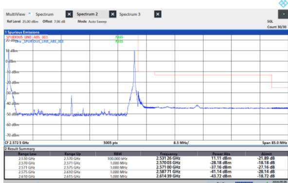
7-7-20MHz-20MHz-64QAM-64QAM-20850-21048-21048-100RB#0-100RB#0
