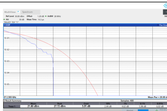
Band41-20MHz-QPSK-41490-100RB#0
