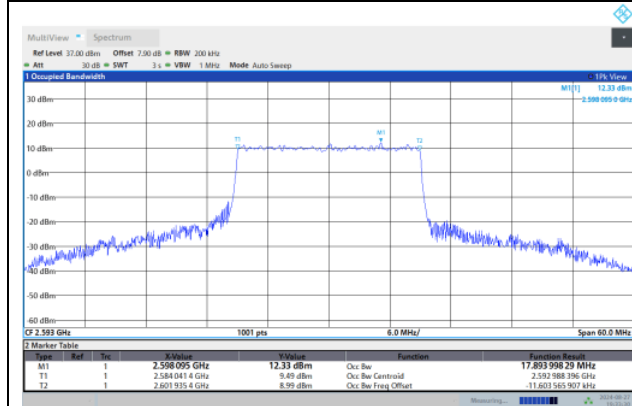
Band41-20MHz-64QAM-40620-100RB#0
