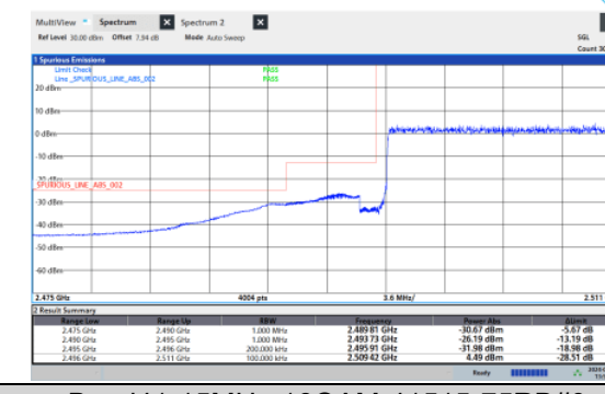
Band41-15MHz-16QAM-41515-75RB#0
