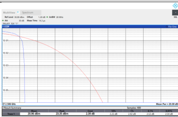
Band41-20MHz-16QAM-40620-1RB#0
