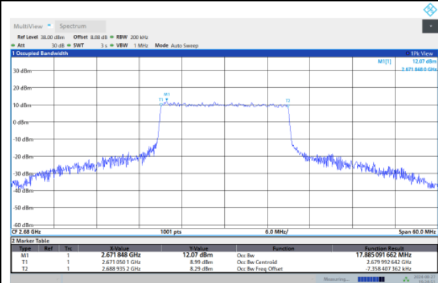
Band41-20MHz-64QAM-41490-100RB#0
