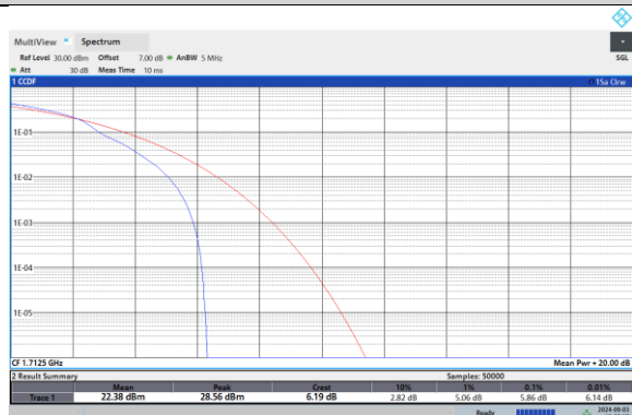
Band66-5MHz-16QAM-132322-1RB#0
