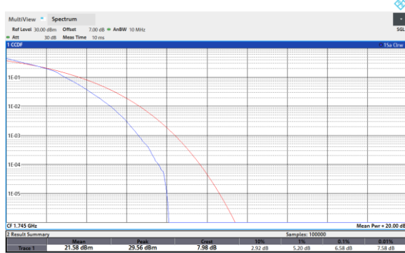
Band66-10MHz-16QAM-132622-50RB#0
