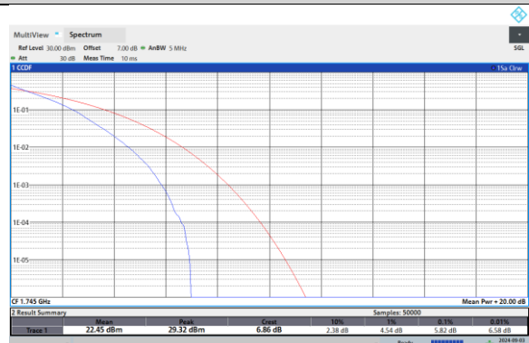
Band66-5MHz-QPSK-132647-25RB#0
