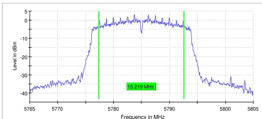
6 dB Bandwidth
