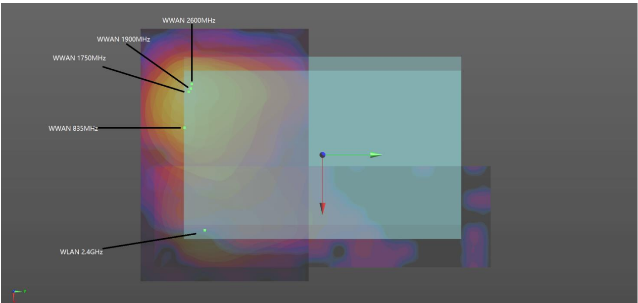
WWAN+WLAN2.4G _Bottom Face 0mm
