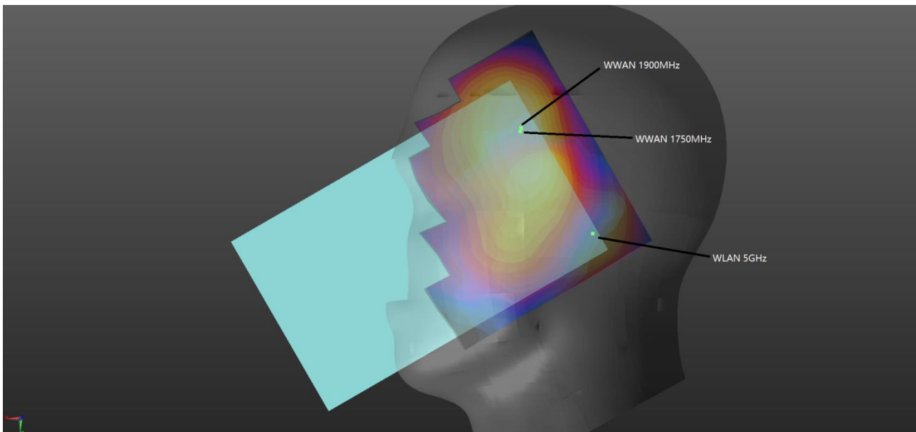
WWAN+WLAN5G _Right Cheek 0mm
