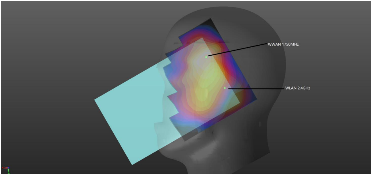
WWAN+WLAN2.4G _Right Cheek 0mm
