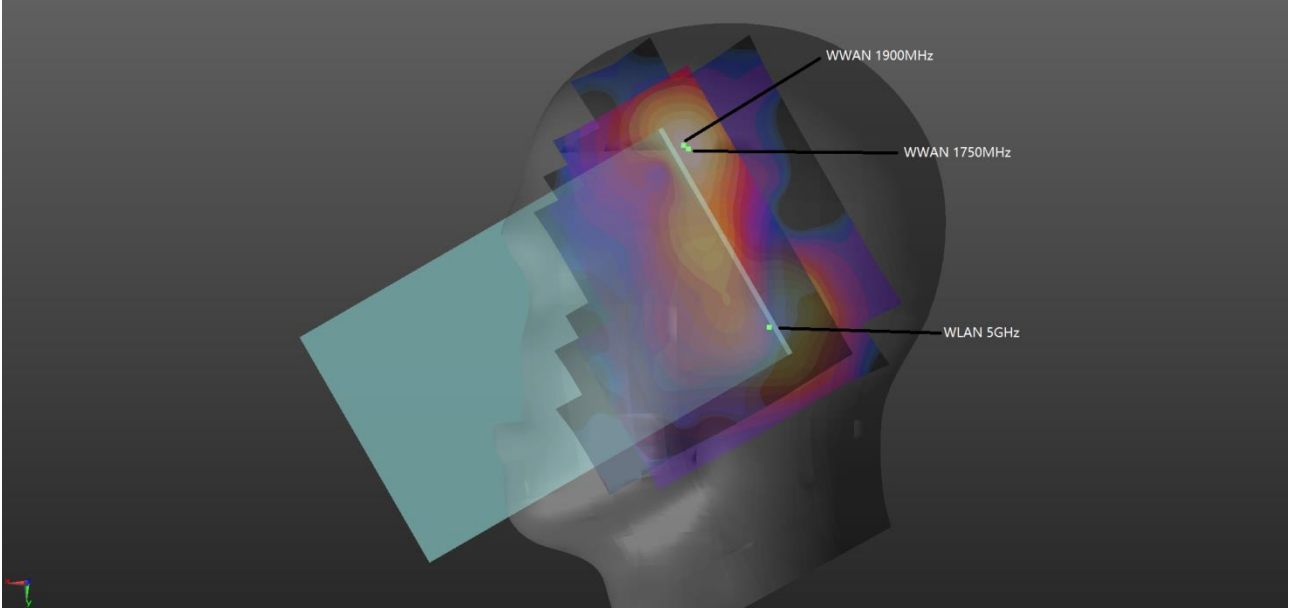
WWAN+WLAN5G _Right Tilted 0mm
