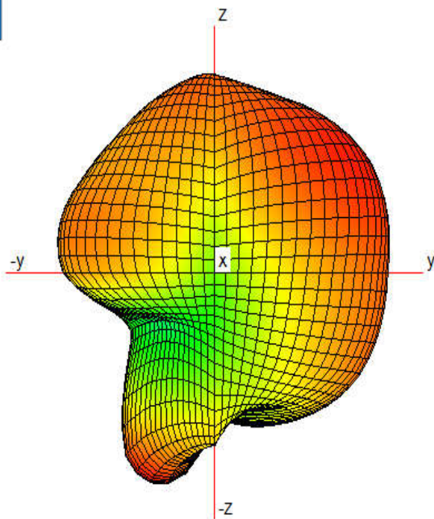
WIFI 5800MHz
