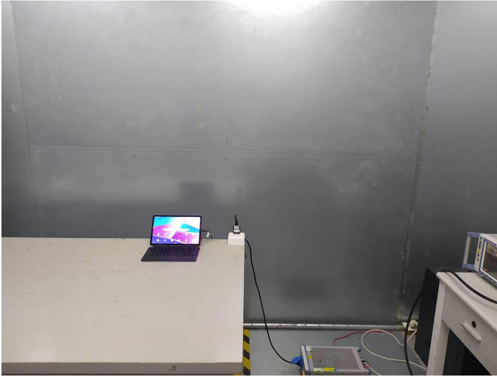
Fig. 3 Power line conducted emission setup photo
