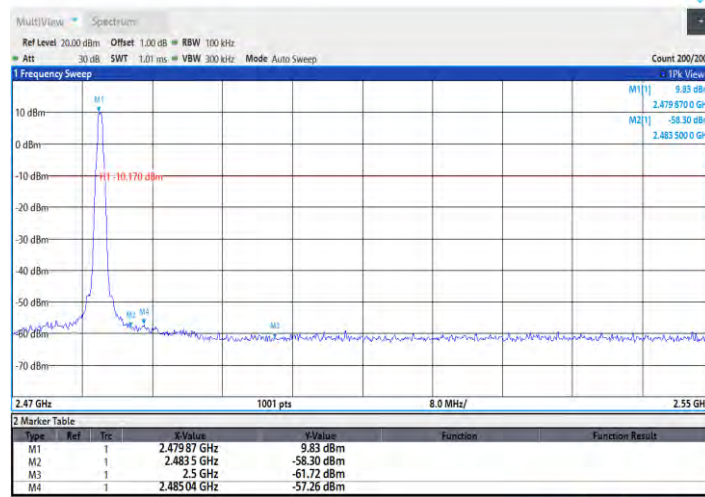
DH5_Ant1_High_2480
