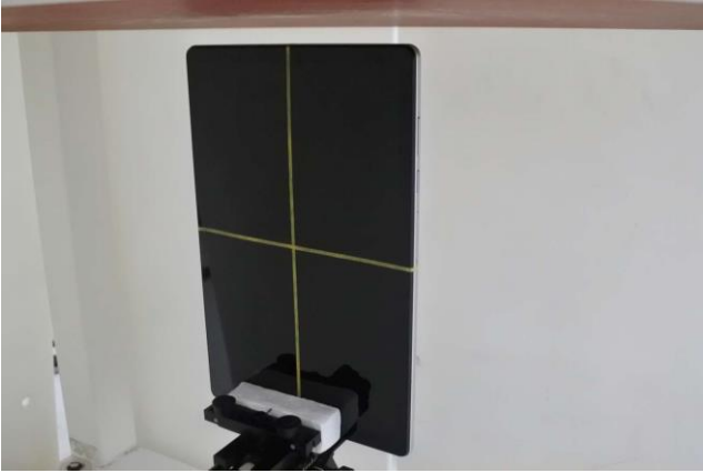
Edge 1 of EUT with Phantom 13 mm Gap (Sensor off)
