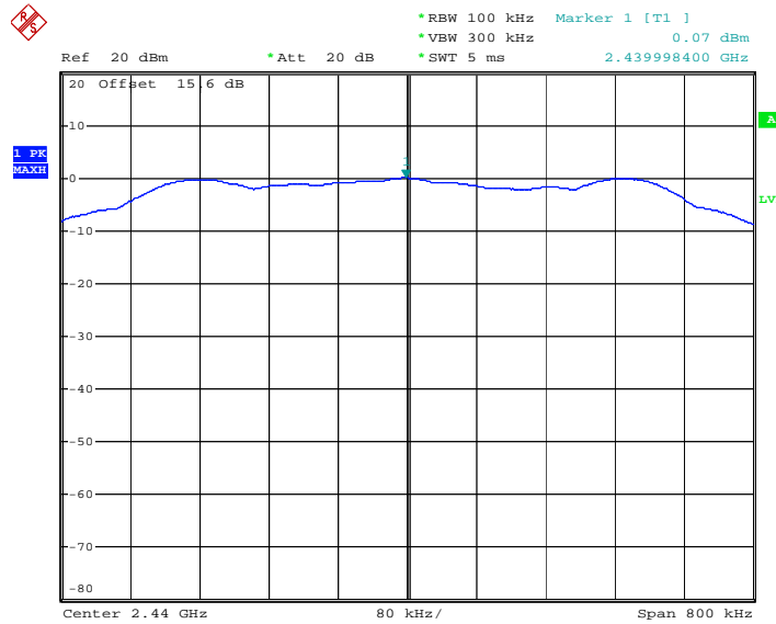
PSD 100kHz Plot on Channel 19
