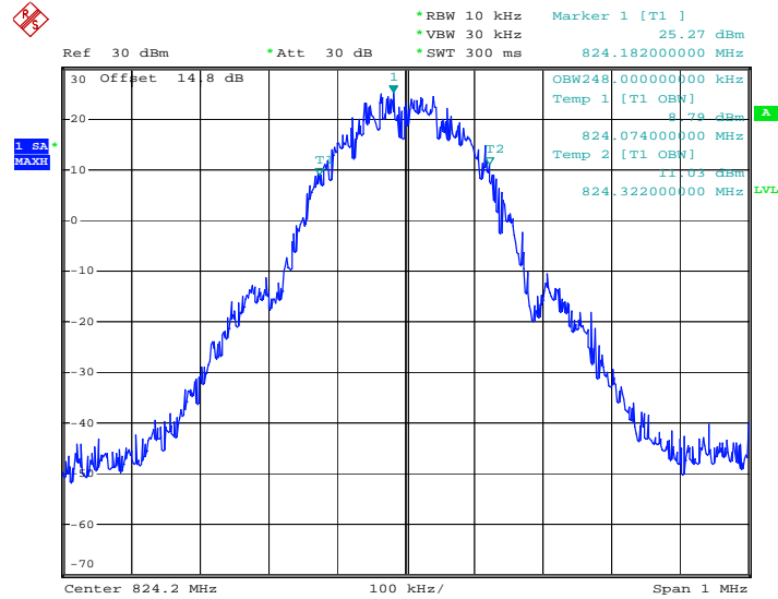
99% Occupied Bandwidth Plot on Channel 128 (824.2 MHz)
