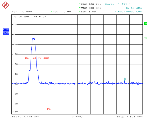
High Band Edge Plot on Channel 39
