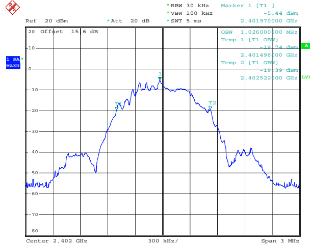
99% Bandwidth Plot on Channel 00
