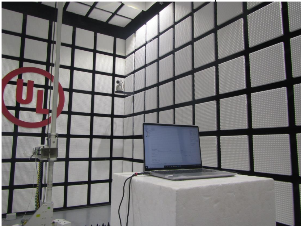
Radiated RF Measurement Setup
