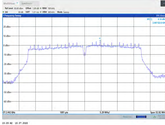
11N40SISO_Ant7_2447
