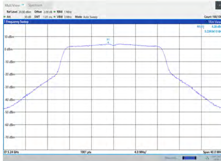
11AC20SISO_Ant7_5240
