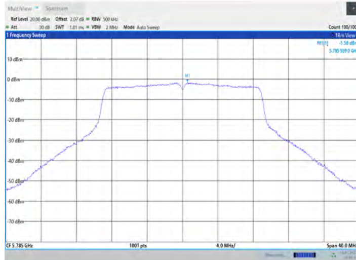
11AC20SISO_Ant7_5785
