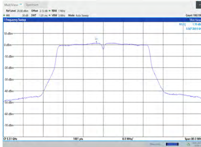
11AC40SISO_Ant7_5510
