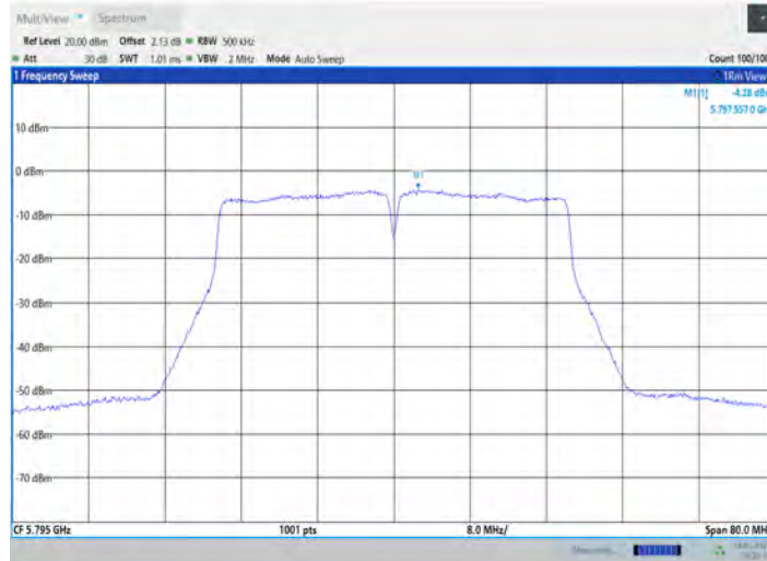
11AC40SISO_Ant7_5795
