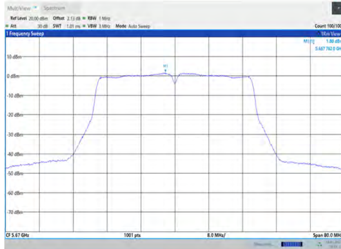
11AC40SISO_Ant7_5670
