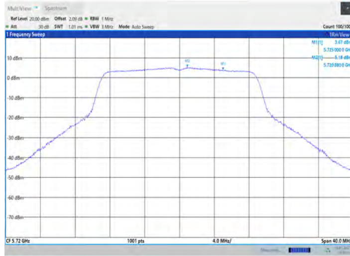
11AC20SISO_Ant7_5720_UNII-3
