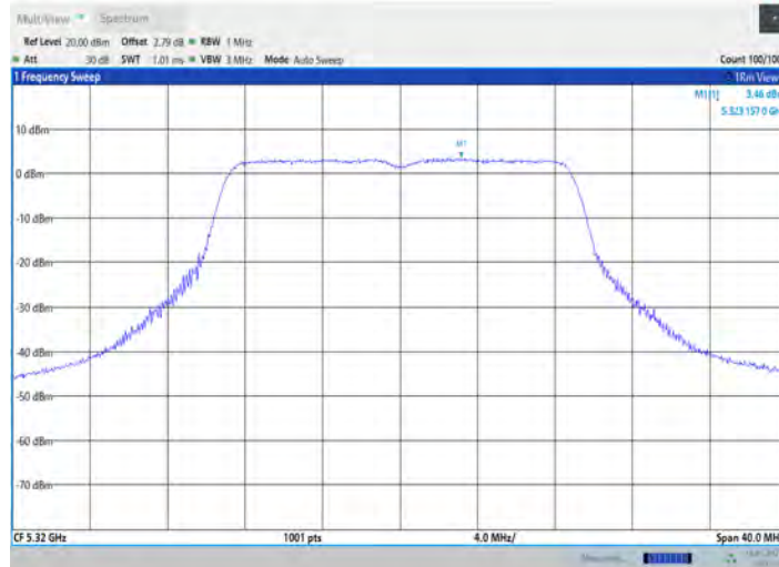
11N20SISO_Ant7_5320
