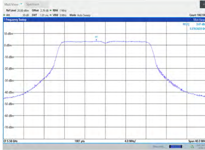
11N20SISO_Ant7_5580
