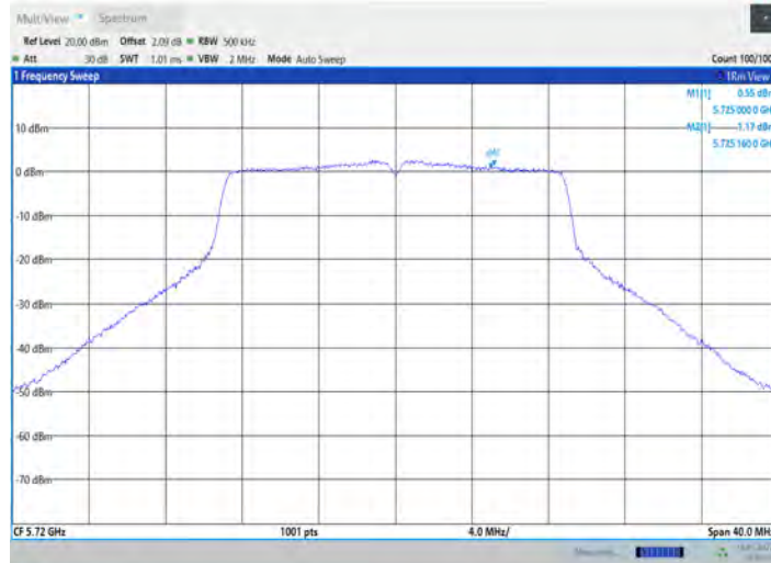
11AC20SISO_Ant7_5720_UNII-3
