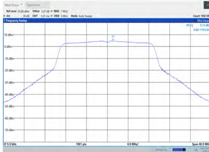
11AC20SISO_Ant7_5500
