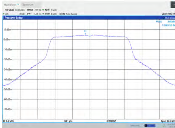
11AC20SISO_Ant7_5300
