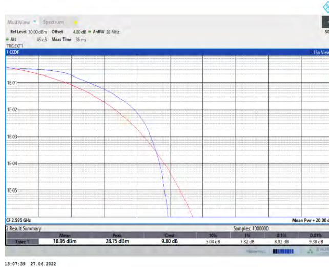
Band38-20MHz-QPSK-38000-100RB#0
