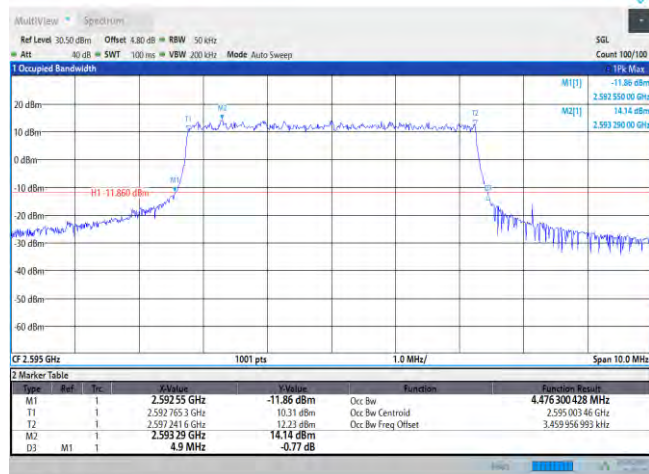
Band38-5MHz-QPSK-38000-25RB#0
