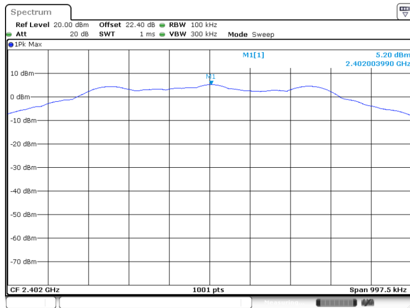
PSD 100kHz Plot on Channel 00_1Mbps
