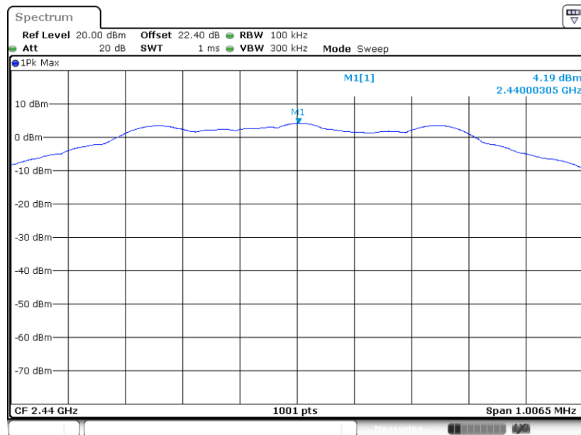
PSD 100kHz Plot on Channel 19_1Mbps
