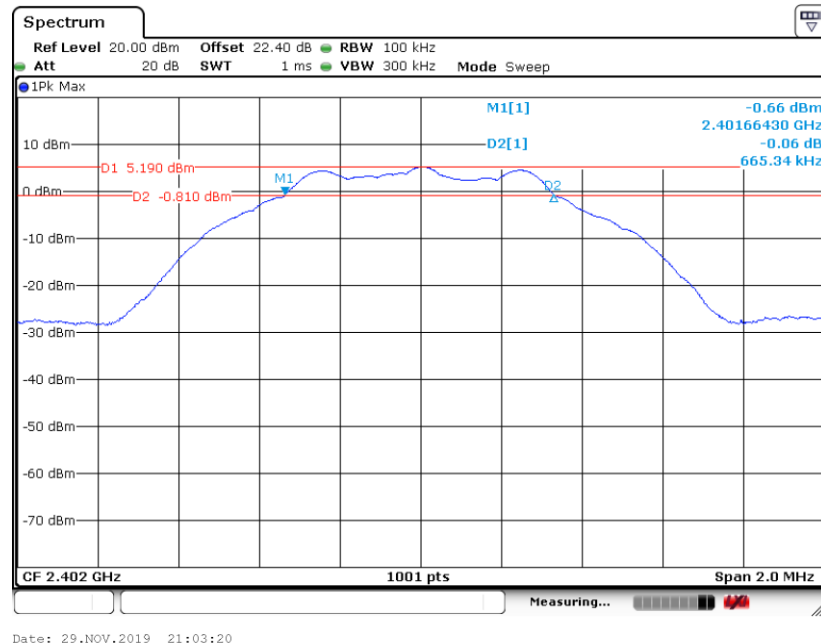
6 dB Bandwidth Plot on Channel 00_1Mbps
