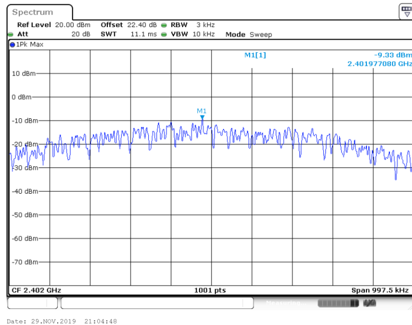
PSD 3kHz Plot on Channel 00_1Mbps
