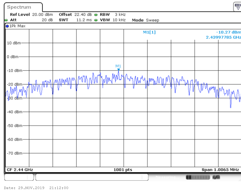
PSD 3kHz Plot on Channel 19_1Mbps
