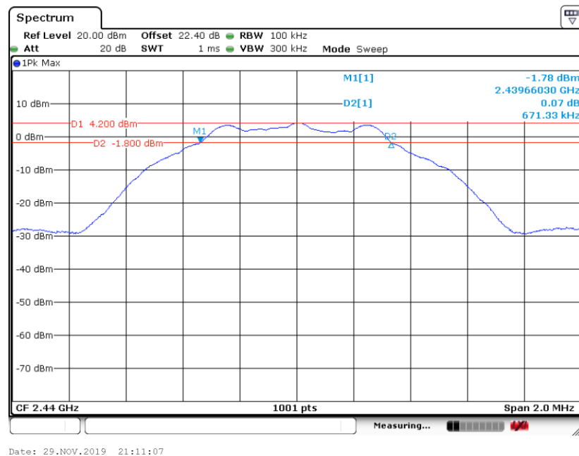
6 dB Bandwidth Plot on Channel 19_1Mbps
