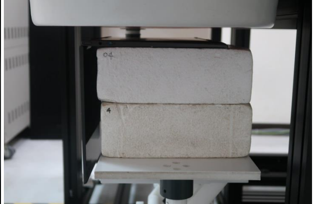
Bottom of Laptop, Test Separation 20 mm
