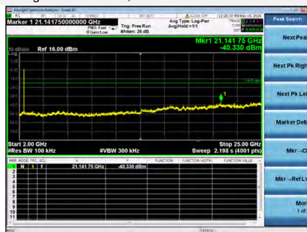
802.11g 12 CHANNEL, SPURIOUS 2 GHz ~ 25 GHz
