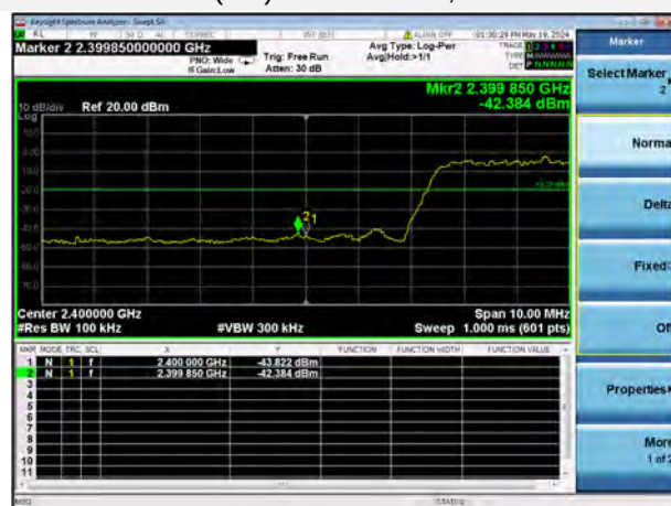
802.11ax-20 MHz(SU) 1 CHANNEL, BAND EDGE
