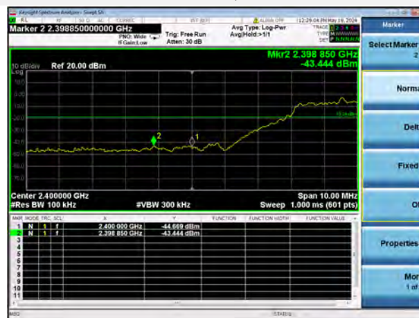
802.11n-20 MHz 1 CHANNEL, BAND EDGE
