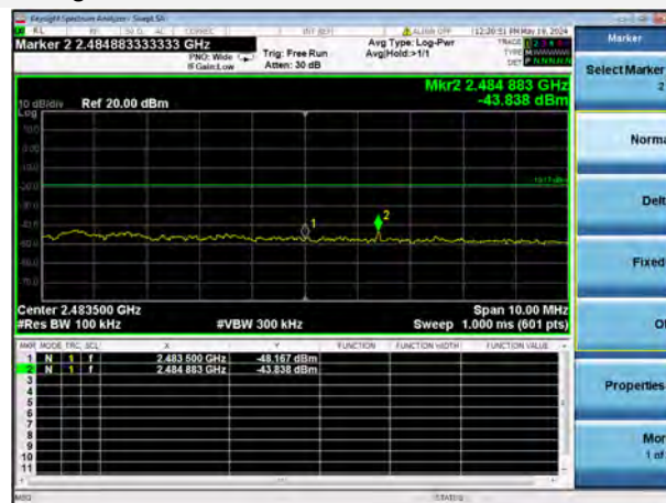
802.11g 12 CHANNEL, BAND EDGE
