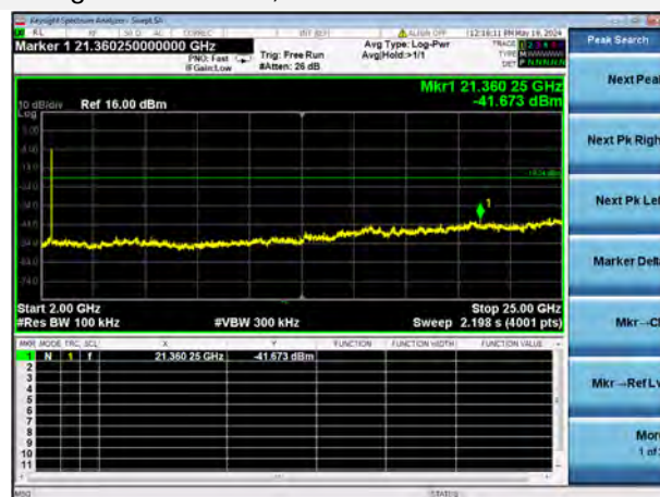
802.11g 11 CHANNEL, SPURIOUS 2 GHz ~ 25 GHz
