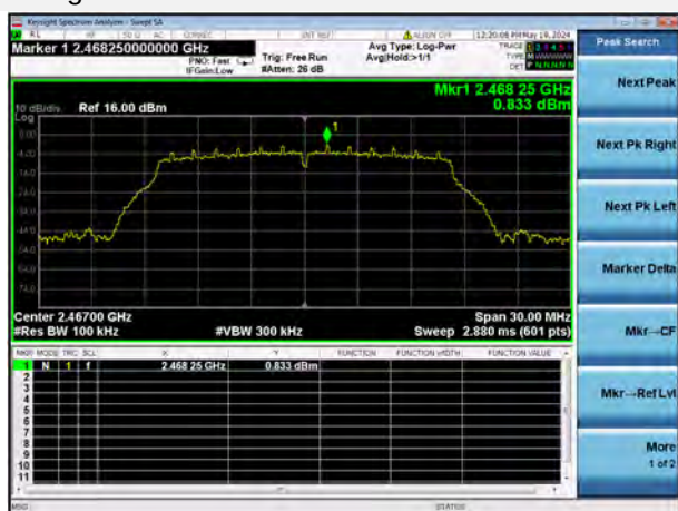
802.11g 12 CHANNEL CARRIER LEVEL
