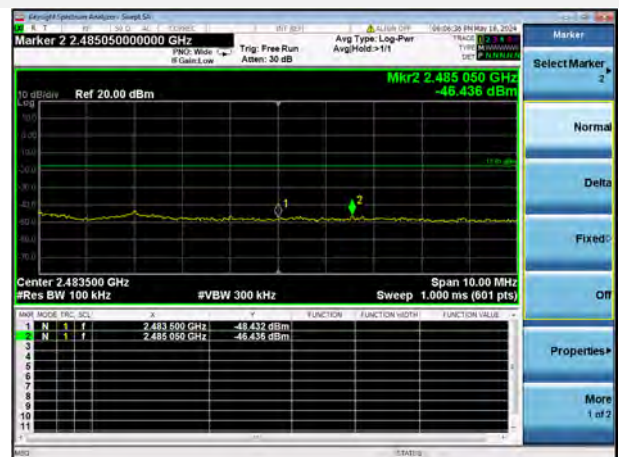
802.11b 12 CHANNEL, BAND EDGE
