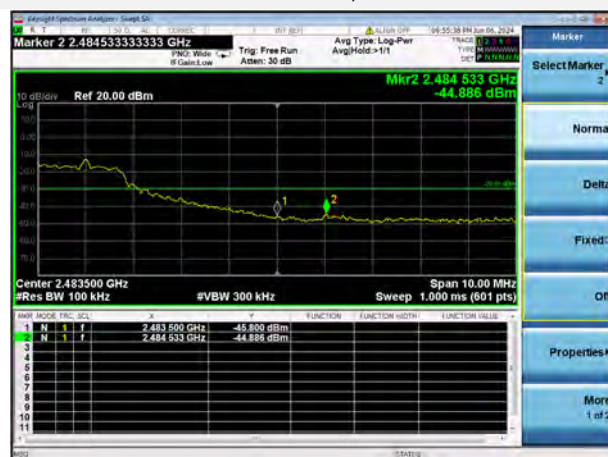
802.11n-40 MHz 11 CHANNEL, BAND EDGE
