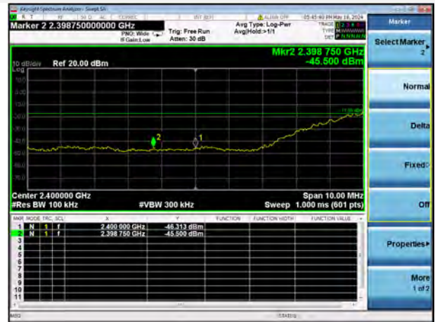
802.11b 1 CHANNEL, BAND EDGE
