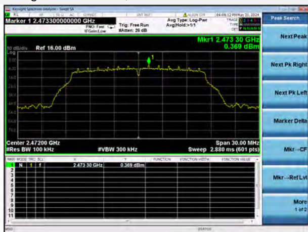
802.11g 13 CHANNEL, CARRIER LEVEL
