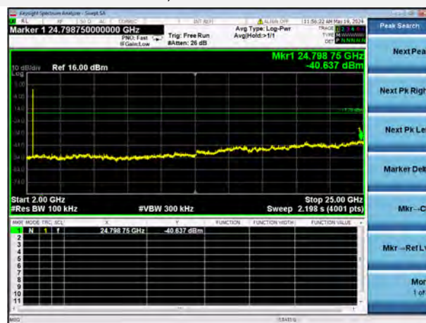
802.11b 6 CHANNEL, SPURIOUS 2 GHz ~ 25 GHz
