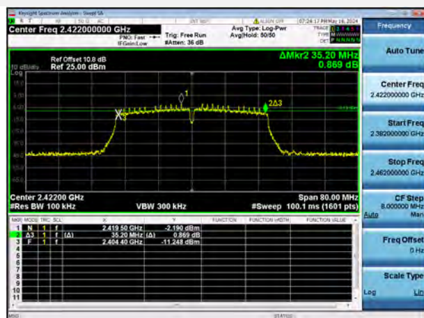
802.11n-40 MHz 3 CHANNEL
