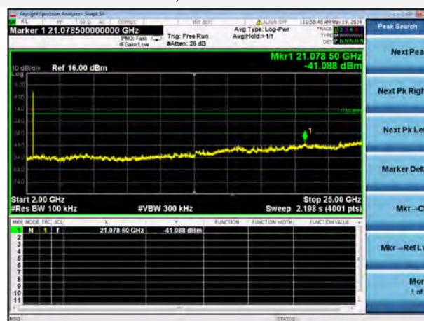
802.11b 11 CHANNEL, SPURIOUS 2 GHz ~ 25 GHz
