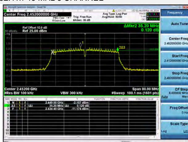
802.11n-40 MHz 9 CHANNEL
