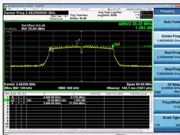
802.11n-40 MHz 11 CHANNEL
