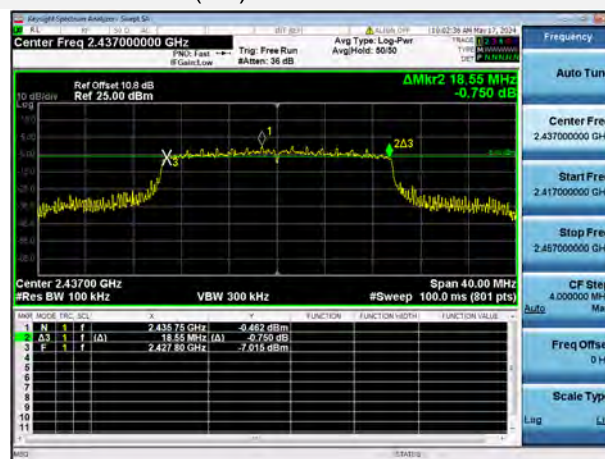
802.11ax-20 MHz(SU) 6 CHANNEL
