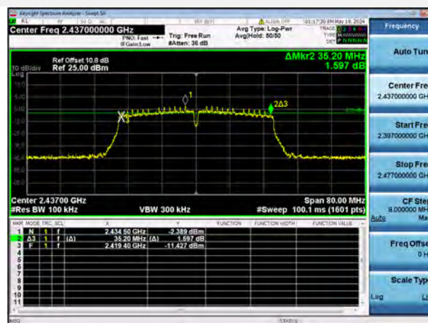
802.11n-40 MHz 6 CHANNEL
