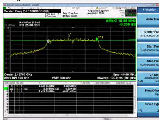
802.11g 6 CHANNEL
