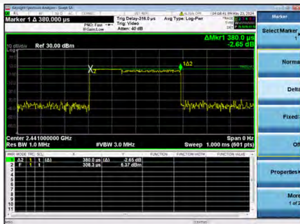
8-DPSK 3DH1
