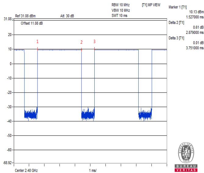
Time-domain plot for Bluetooth transmission signal
