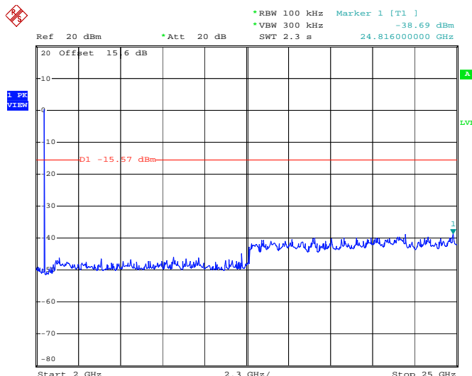
Conducted Spurious Emission Plot between 2 GHz ~ 25 GHz
