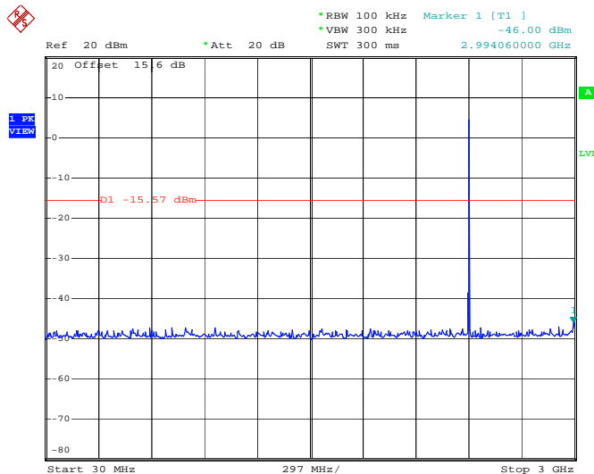
Conducted Spurious Emission Plot between 30MHz ~ 3 GHz
