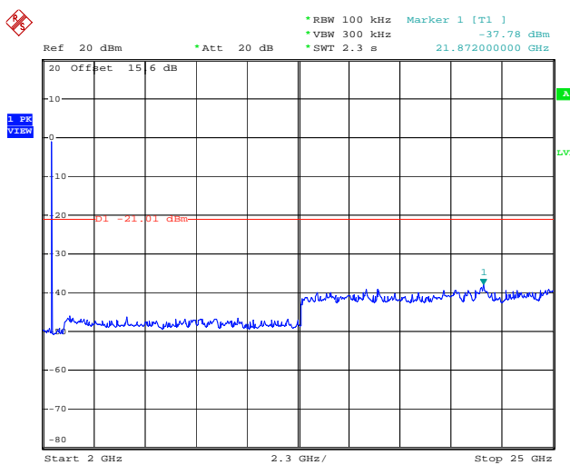
Conducted Spurious Emission Plot on Bluetooth 4.0 - LE 1Mbps GFSK Channel 00
