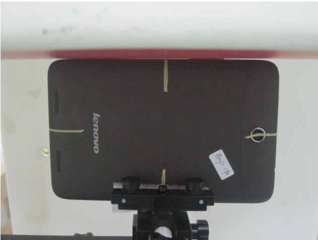
Primary Portrait of the DUT with Phantom 0 cm Gap
