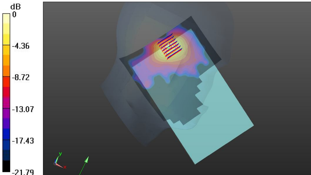
0 dB = 0.672 \text{ W/kg}
