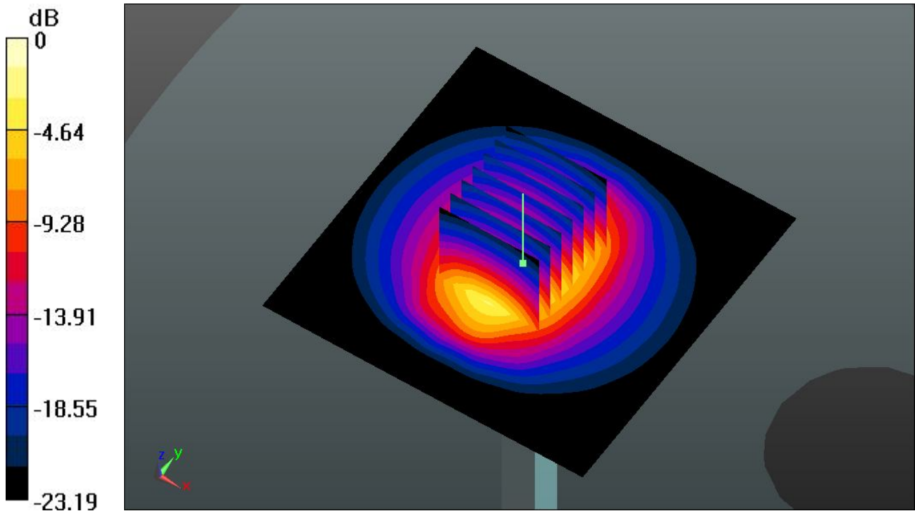
0 dB = 22.3 \text{ W/kg}
