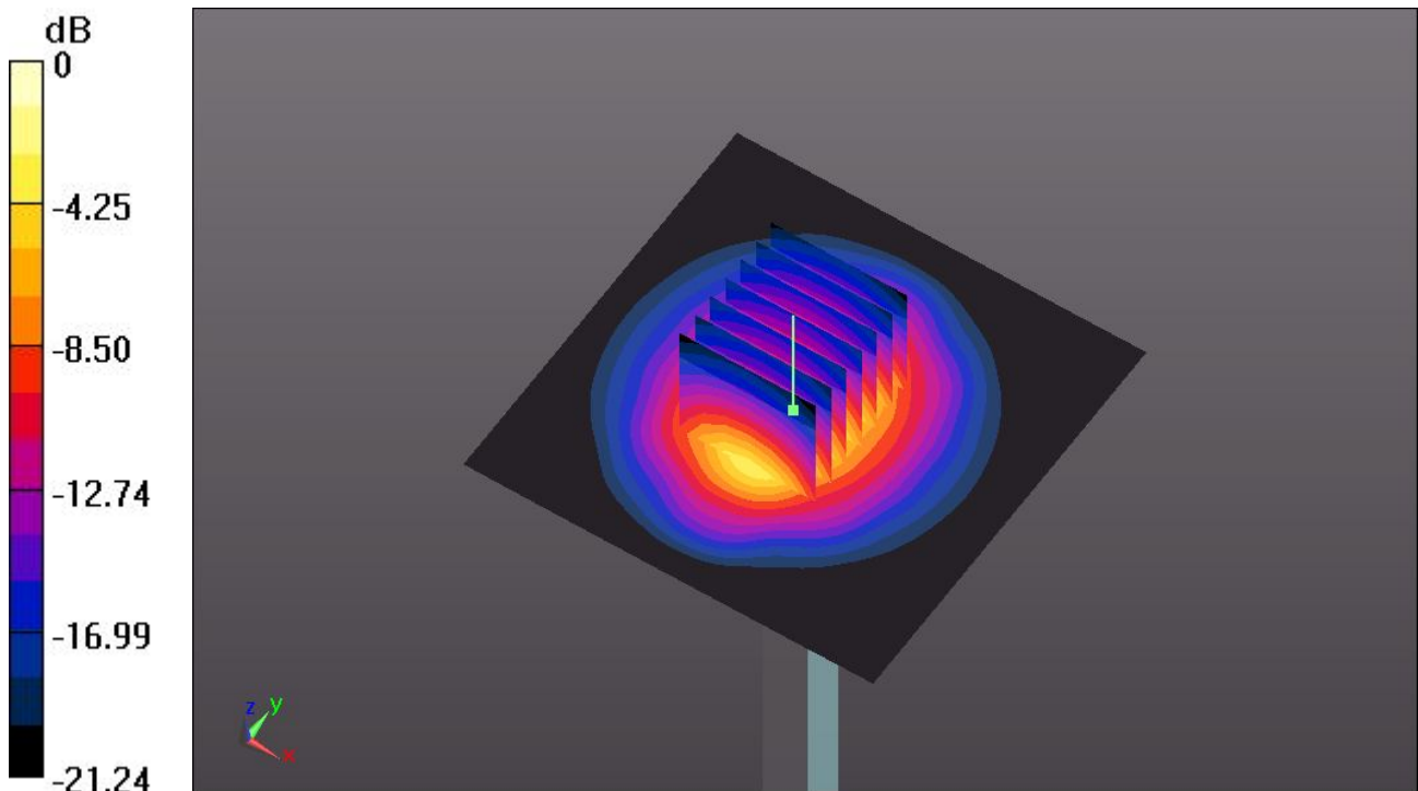
0 dB = 14.1 \text{ W/kg}
