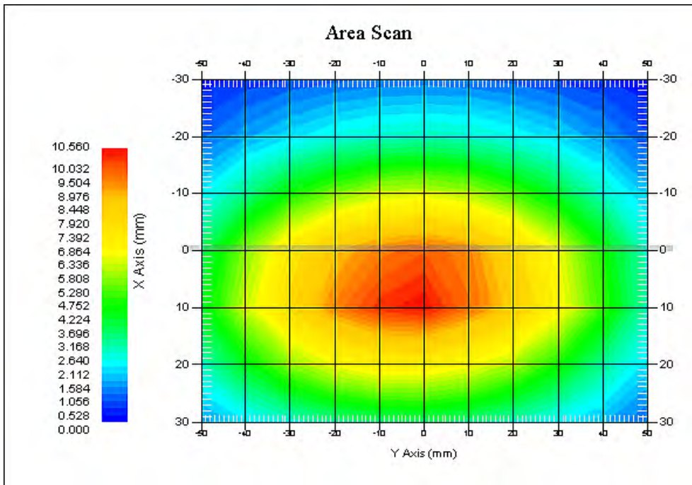
835 MHz System Validation with Head Tissue
